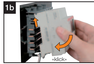
SMISLINE TP mounting
