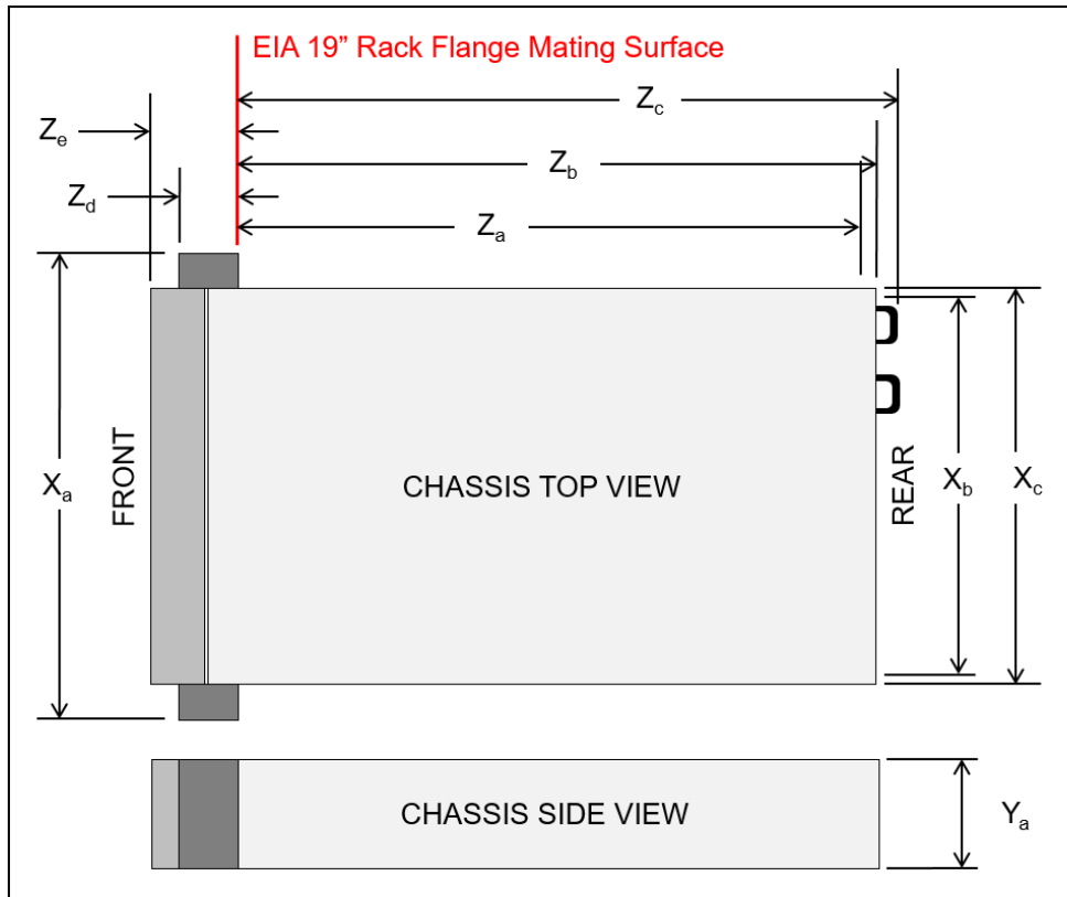
Figure 27. Server dimensions
