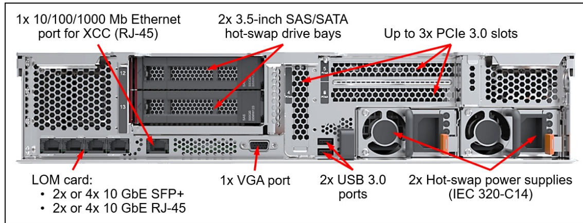
Figure 4. VX5520 rear view with rear drive bays
