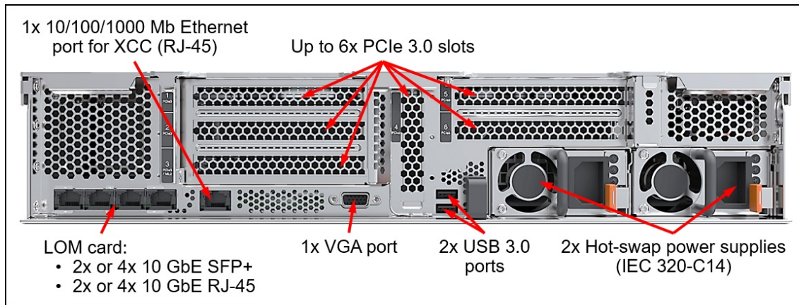
Figure 3. VX5520 rear view without rear drive bays
