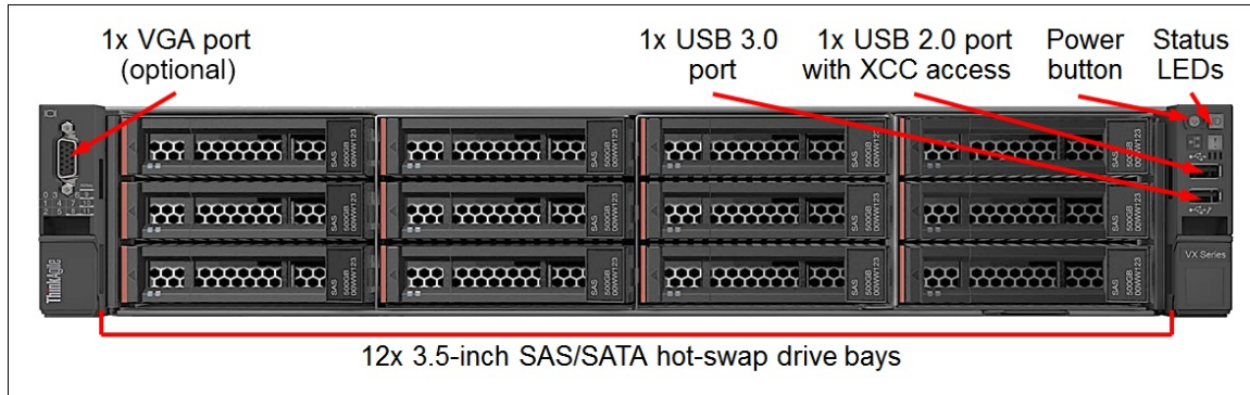
Figure 2. VX5520 front view
