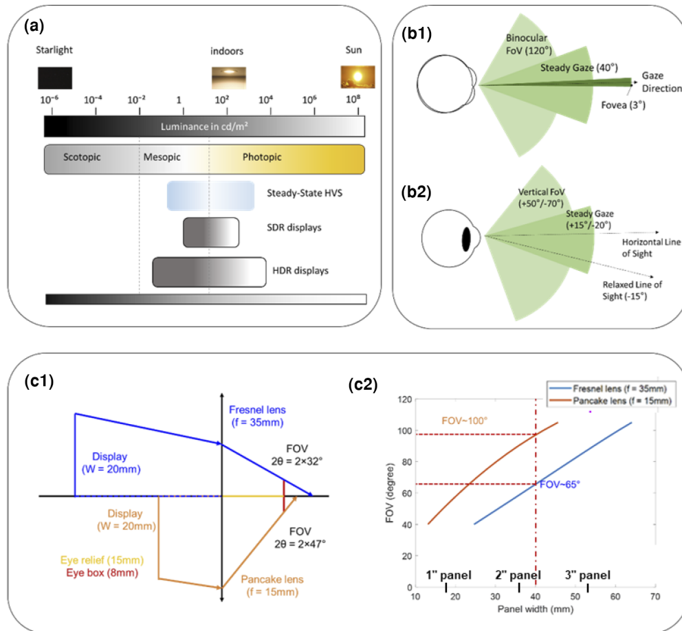
(a) Dynamic range of the human visual system. (b1) Horizontal human vision FoV. (b2) Vertical human vision FoV. (c1) Schematics of FoV calculations in Fresnel and pancake VR systems at a given display panel width, eye relief, and eyebox, assuming the optical power is provided by a singlet lens. (c2) Relation between FoV and panel width in Fresnel- and pancake-lens-based VR systems.
