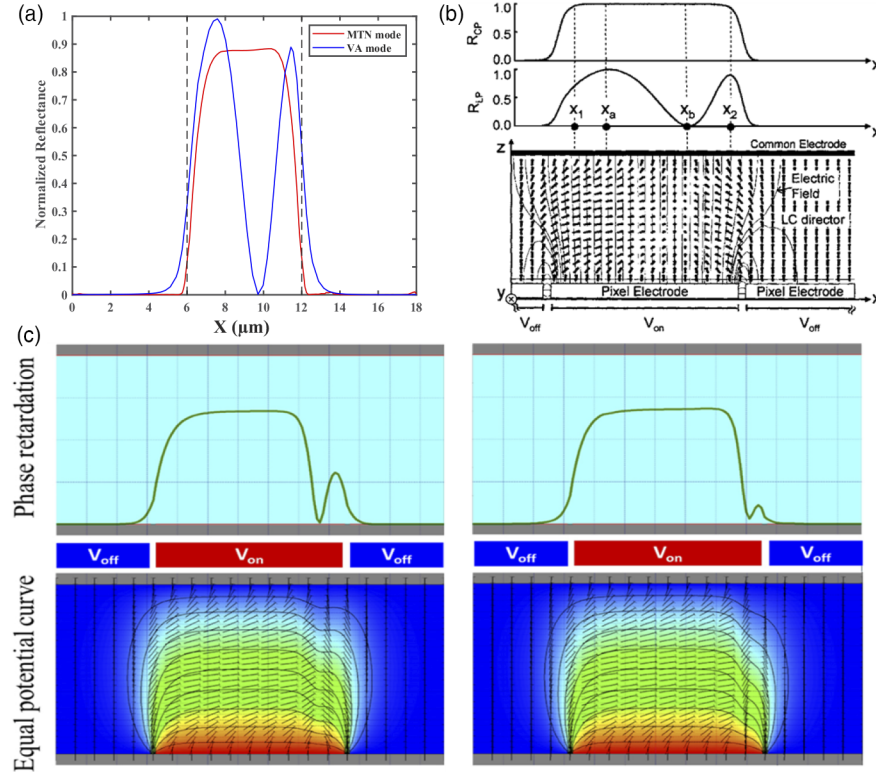
(a) Simulated FFE of the MTN and VA modes in an amplitude LCOS device and (b) CP light employed to eliminate the FFE of the VA modes. Reprinted with permission from Chiang et al. , Appl. Phys. Lett. 87 , 031110 (2005) [136]. Copyright 2005, AIP Publishing LLC. (c) FFE without patterned pretilt angle (left) and the reduced FFE with patterned pretilt angle (right). Reprinted from [132] under a Creative Commons license .
