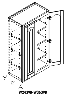
W2439B-W3639B
