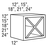
WSC121212-WSC242412
