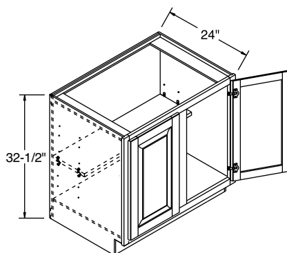
B39FH32.5-B48FH32.5
