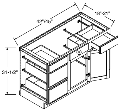
VBB4218D-VBB4518D L or R VBB42D-VBB45D L or R 6 drawers
