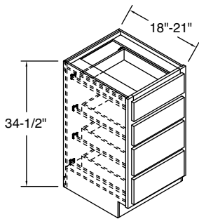
4VBD1218BH-4VBD2418BH 4VBD12BH-4VBD24BH
