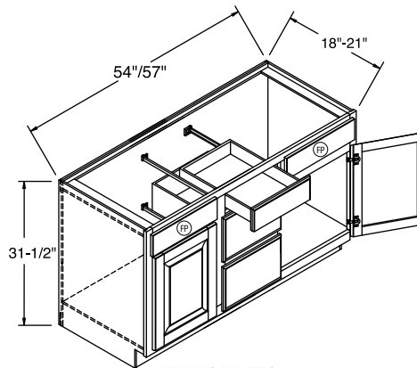
VDB5418-VDB5718 VDB54-VDB57
