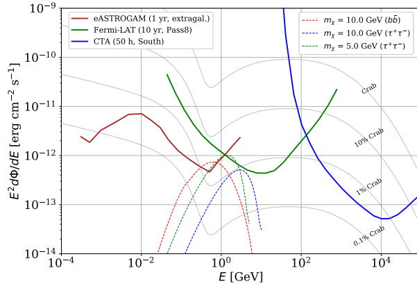
Figure 4.8.1: e-ASTROGAM differential sensitivity (solid brown line) to point-like WIMP DM subhalos, compared to those of the Fermi -LAT (green) and the future CTA (blue). Dashed lines represent examples of DM subhalo energy fluxes for three DM particle models. A J -factor value of 1.5 \times 10^{19} \text{ GeV}^2 \text{ cm}^{-5} and a \langle \sigma_{ann} v \rangle value of 2.2 \times 10^{-26} \text{ cm}^3 \text{ s}^{-1} have been assumed. See text for further details.
