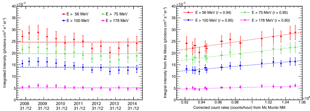
Figure 7.3.1: Left: time evolution of the lunar gamma-ray intensity above 56, 75, 100 and 178 MeV [764]. Right: study of the correlations between the lunar gamma-ray intensity [764] and the count rates of the McMurdo neutron monitor [770]. The values reported in brackets are the correlation coefficients.
