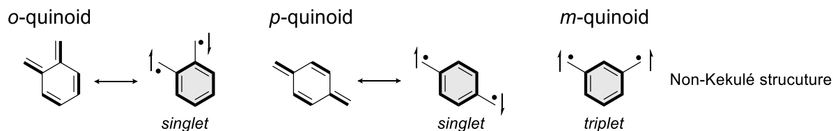
Figure 3. Quinoidal structures.
