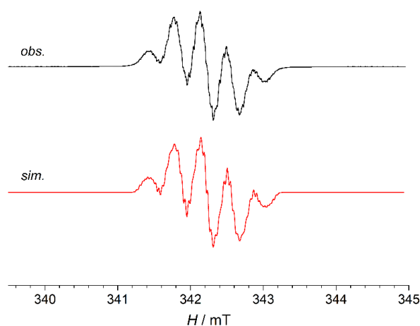
Figure S2. ESR spectrum of a \text{CH}_2\text{Cl}_2 solution of \mathbf{1c}^{\bullet+}\cdot\text{SbF}_6^- at 295 K. 9.59252 GHz, g -value = 2.00260, Gain = 22500, sweep time = 3.4 min, modulation amplitude = 0.01 mT.
