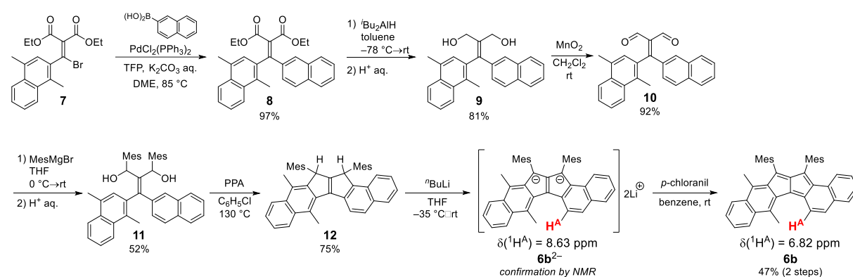
Scheme 1. Synthetic route for 6b . TFP = tri(2-furyl)phosphine, Mes = 2,4,6-trimethylphenyl, PPA = polyphosphoric acid.
