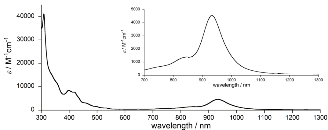
Figure S11. Electronic absorption spectrum of 1b in CH 2 Cl 2 . Inset shows a magnified view.
