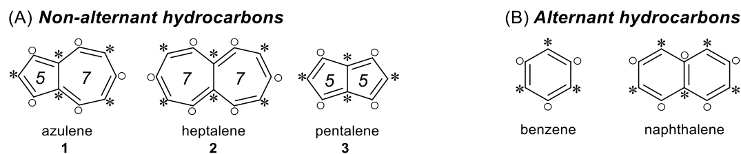
Figure 1. Examples of (A) non-alternant and (B) alternant hydrocarbons.
