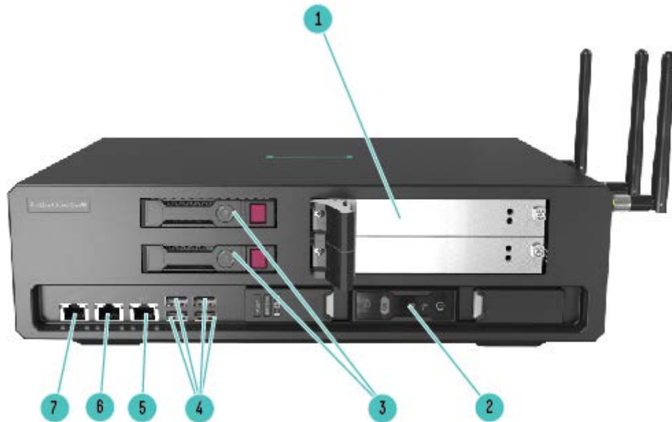
HPE Edgeline EL1000 Front View
