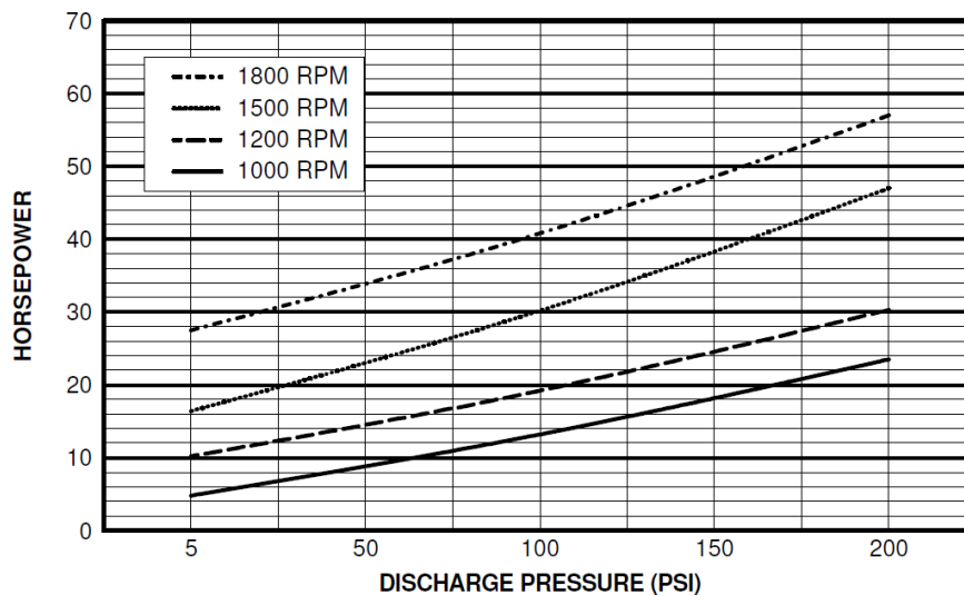
PUMP WATER HP VERSUS DISCHARGE PRESSURE EDWARDS MODEL 300-368 SD / 300-368 SDF
