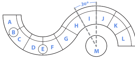
Example Steps Lounge configuration plan
