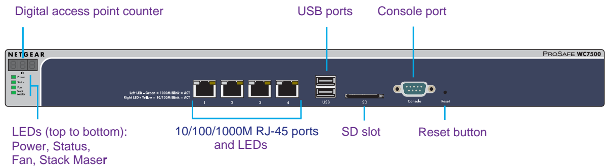
Figure 1. Front panel models WC7500 and WC7600v2
