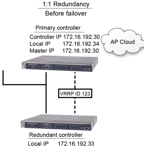
Figure 19. Primary and redundant controllers before a failover
