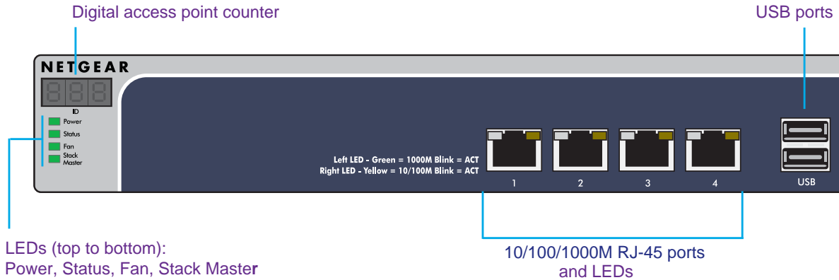
Figure 2. Front panel close-up models WC7500 and WC7600v2
