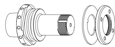
GWA HSK-E50 // \varnothing 31,75 mm ( 1\frac{1}{4} ) // without RS
