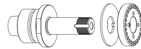
GWA manual HSK-F40 // \varnothing 31,75 mm // without RS
