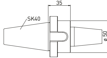
Order No. Name 350130043 Adapter SK40 on Strausak Fleximat
