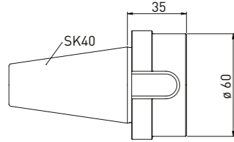
Order No. Name 350130040 Adapter SK40 on Saacke short taper
