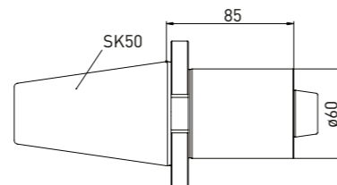
Order No. Name 350130045 Adapter SK50 on Haas/Walter taper L85
