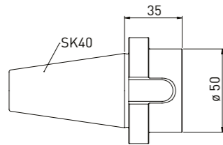
Order No. Name 350130042 Adapter SK40 on Strausak Promat
