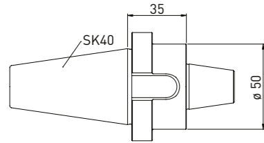
Order No. Name 350130035 Adapter SK40 on ANCA taper \varnothing 30
