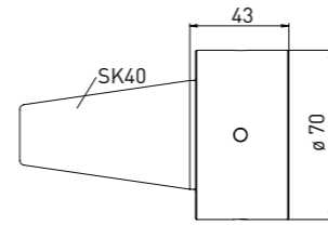
Order No. Name 350130039 Adapter SK40 on Rollomatic \varnothing 25
