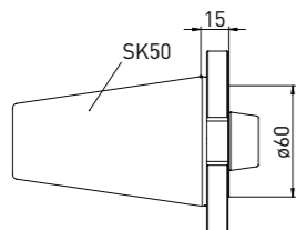
Order No. Name 350130044 Adapter SK50 on Haas/Walter taper L15
