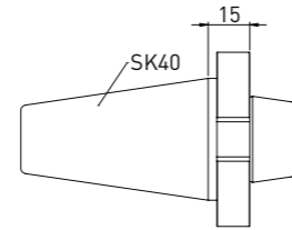
Order No. Name 350130014 Adapter SK40 on Haas/Walter taper
