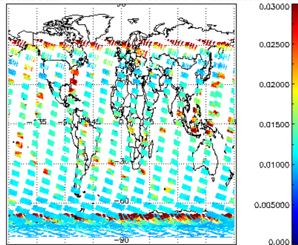
SCIOL2P_NADUV003_vcd_err for 14DEC2003 00:00:00 to 15DEC2003 00:00:00
