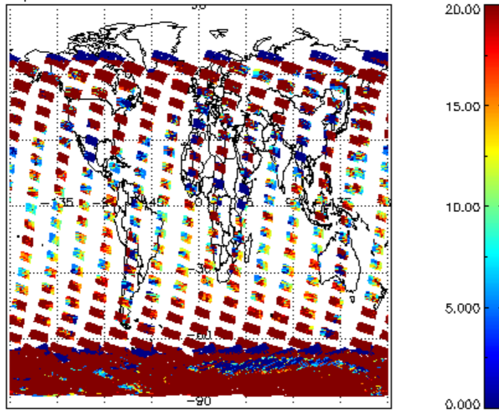
cL_opt_depth for 14DEC2003 00:00:00 to 15DEC2003 00:00:00
