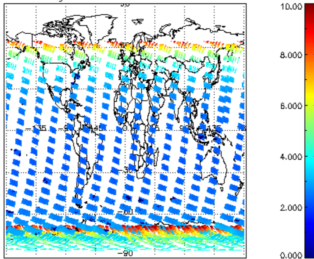
SCIOL2P_NADUV003_amf_gr for 14DEC2003 00:00:00 to 15DEC2003 00:00:00
