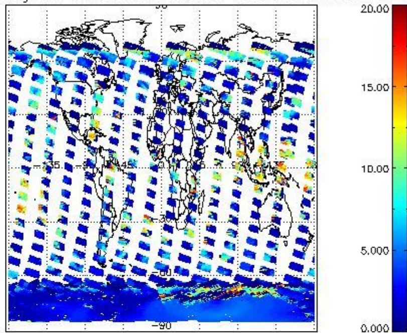
cL_top_height for 14DEC2003 00:00:00 to 15DEC2003 00:00:00
