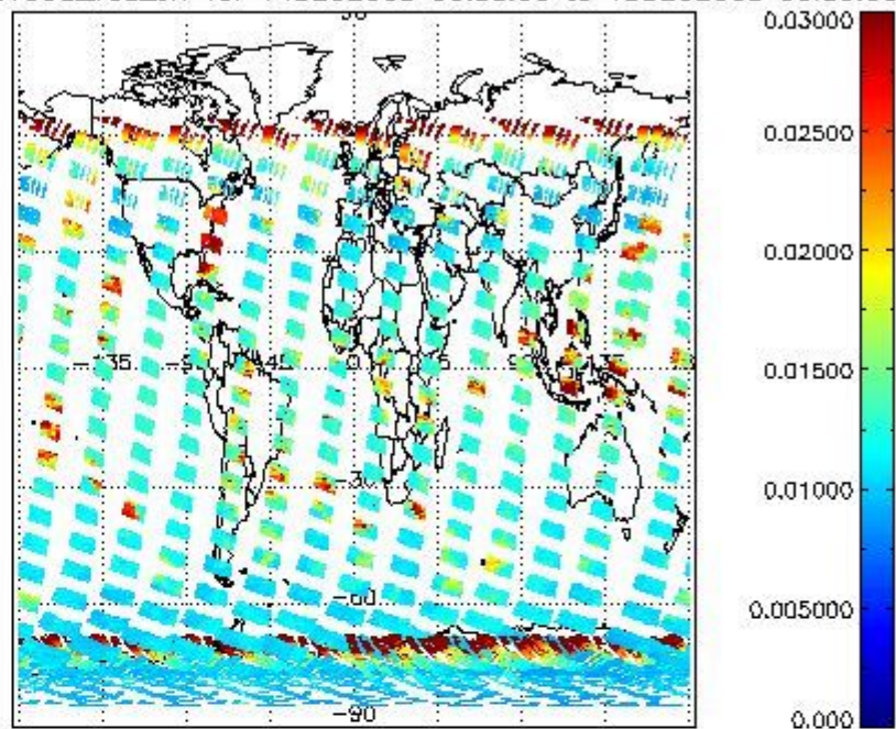
SCIOL2P_NADUV003_vcd_err for 14DEC2003 00:00:00 to 15DEC2003 00:00:00
