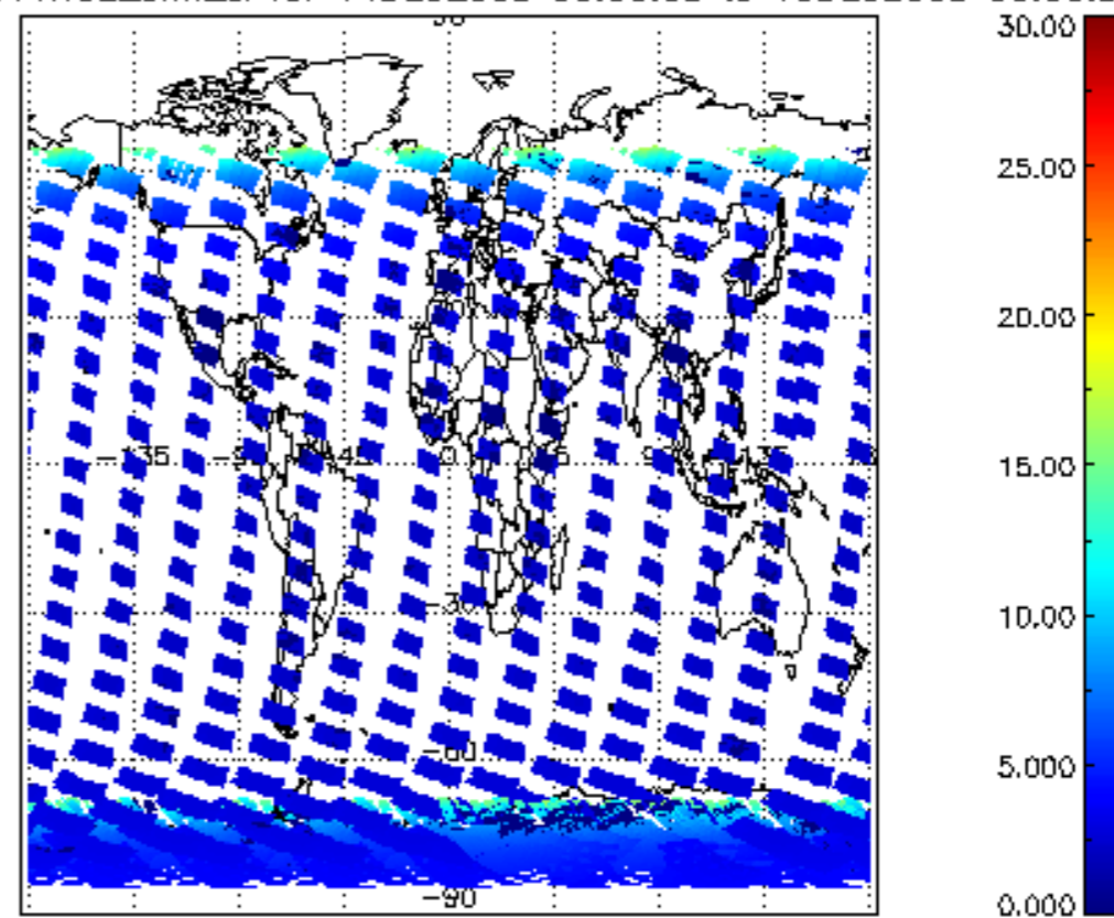
SCIOL2P_NADUV1NO2_amf_cl for 14DEC2003 00:00:00 to 15DEC2003 00:00:00
