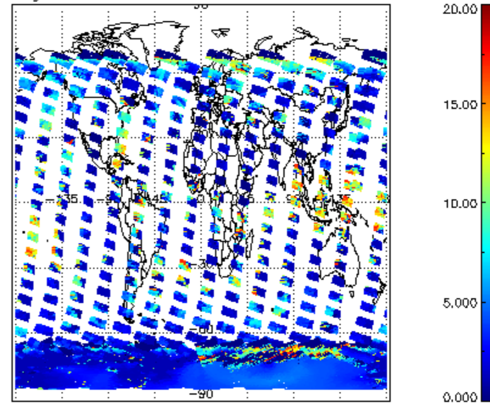
cL_top_height for 14DEC2003 00:00:00 to 15DEC2003 00:00:00
