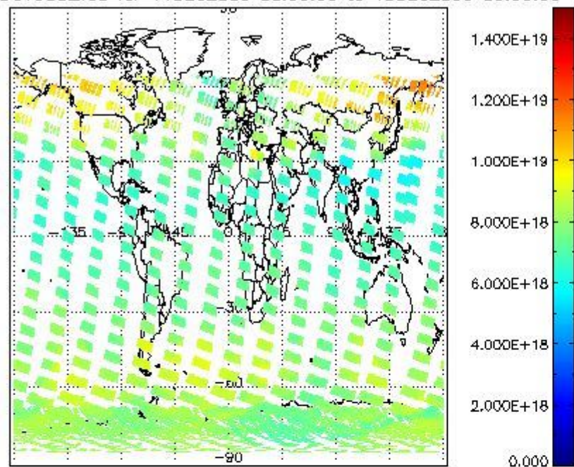
SCIOL2P_NADUV003_vcd for 14DEC2003 00:00:00 to 15DEC2003 00:00:00
