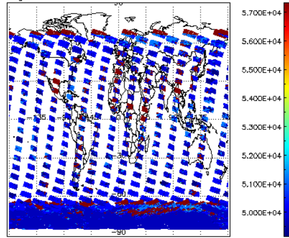
cloud_flags for 14DEC2003 00:00:00 to 15DEC2003 00:00:00
