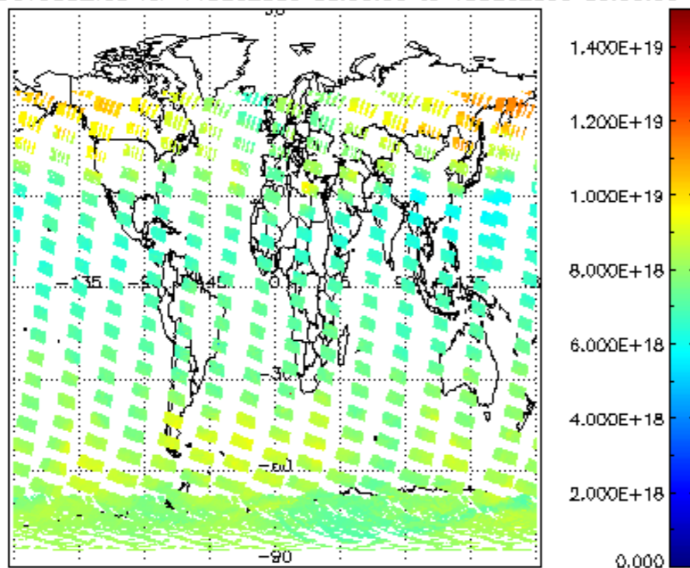
SCIOL2P_NADUV003_vcd for 14DEC2003 00:00:00 to 15DEC2003 00:00:00
