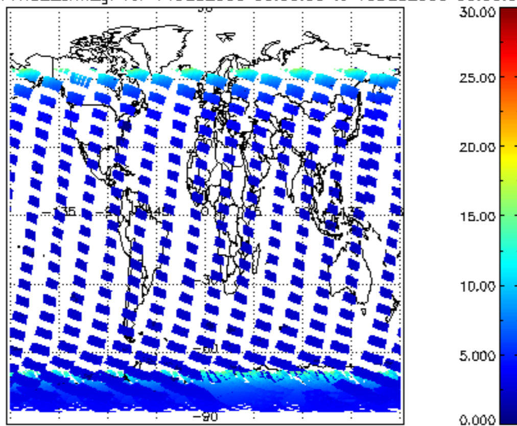
SCIOL2P_NADUV1NO2_amf_gr for 14DEC2003 00:00:00 to 15DEC2003 00:00:00
