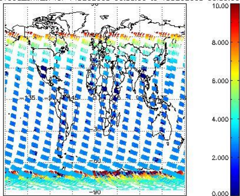
SCIOL2P_NADUV003_amf_cl for 14DEC2003 00:00:00 to 15DEC2003 00:00:00
