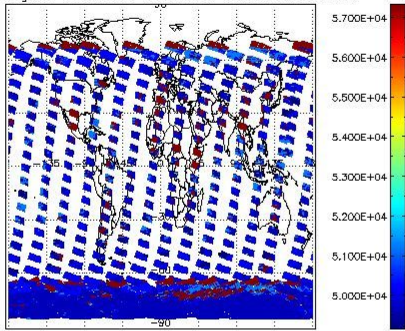
cloud_flags for 14DEC2003 00:00:00 to 15DEC2003 00:00:00
