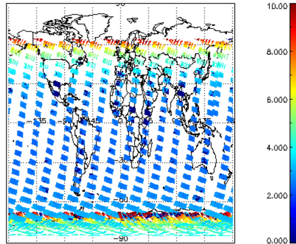
SCIOL2P_NADUV003_amf_cl for 14DEC2003 00:00:00 to 15DEC2003 00:00:00
