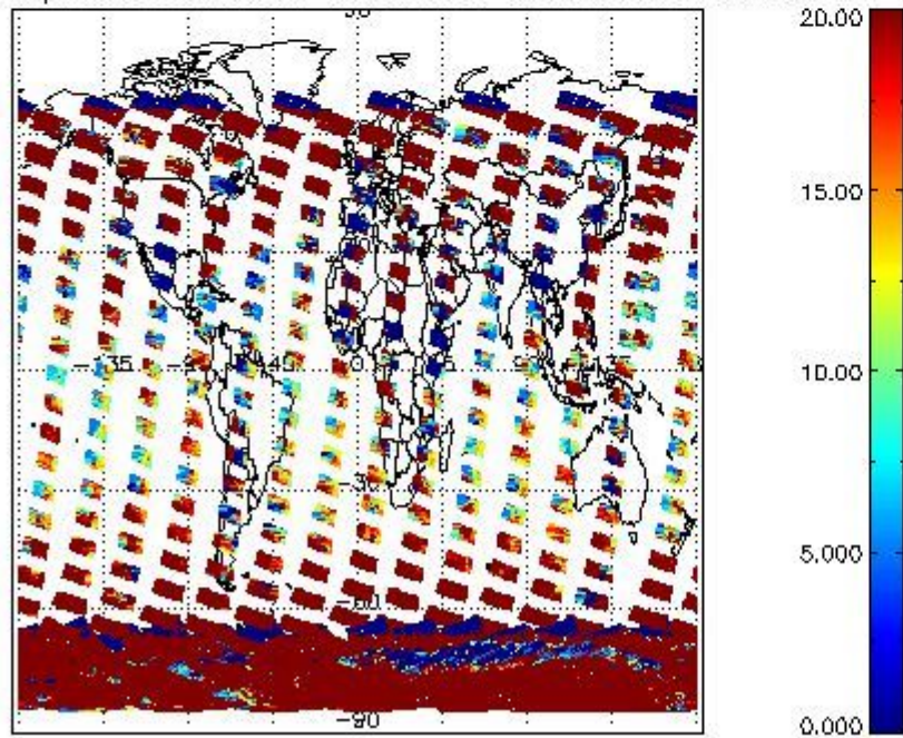
cL_opt_depth for 14DEC2003 00:00:00 to 15DEC2003 00:00:00
