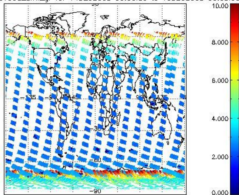
SCIOL2P_NADUV003_amf_gr for 14DEC2003 00:00:00 to 15DEC2003 00:00:00
