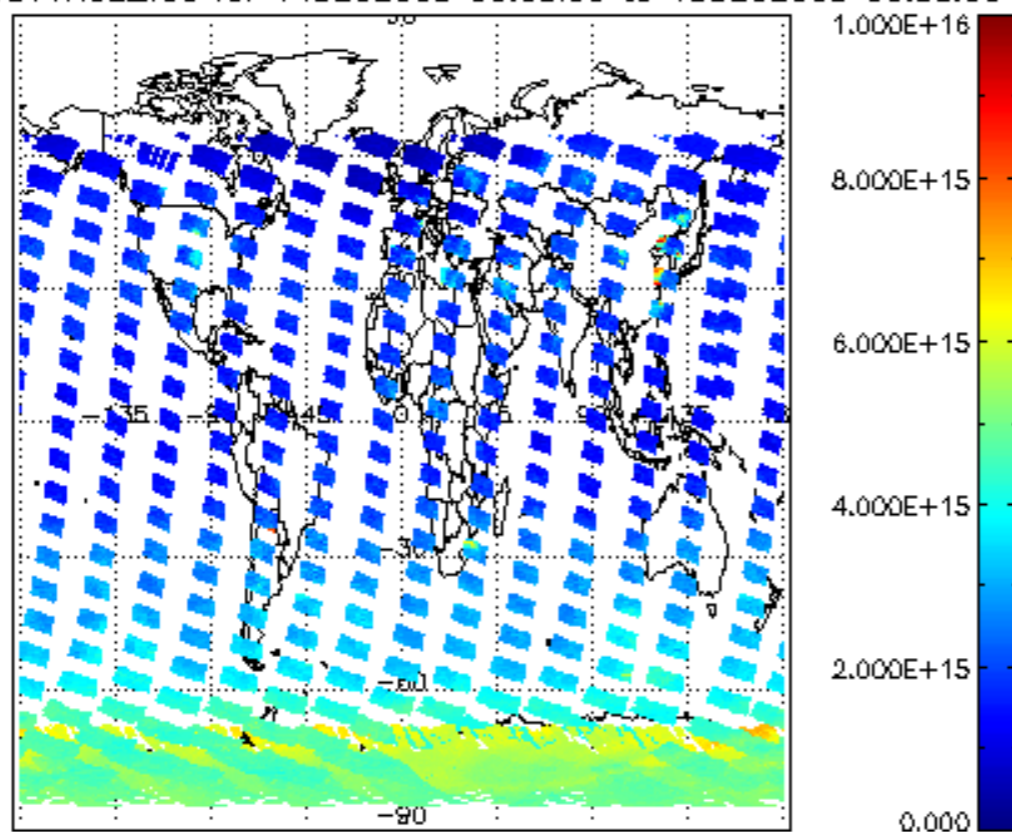
SCIOL2P_NADUV1NO2_vcd for 14DEC2003 00:00:00 to 15DEC2003 00:00:00
