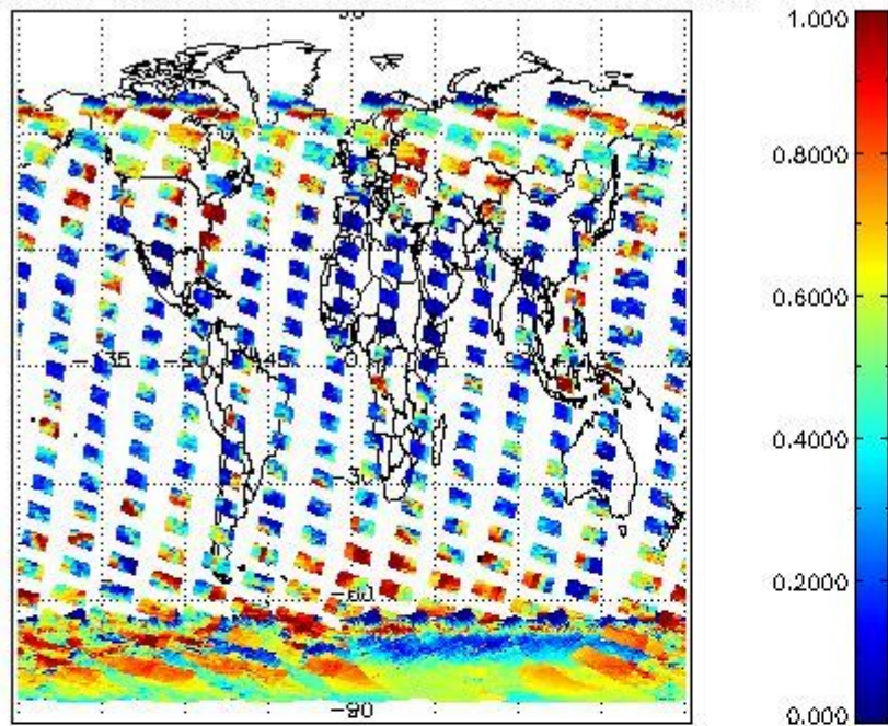
cL_frac for 14DEC2003 00:00:00 to 15DEC2003 00:00:00
