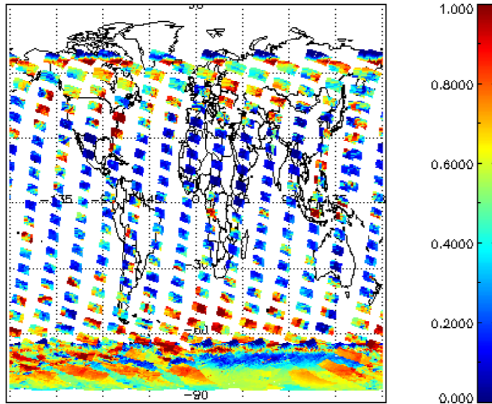
cL_frac for 14DEC2003 00:00:00 to 15DEC2003 00:00:00
