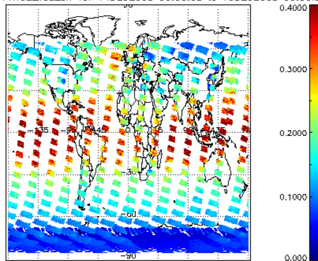
SCIOL2P_NADUV1NO2_vcd_err for 14DEC2003 00:00:00 to 15DEC2003 00:00:00
