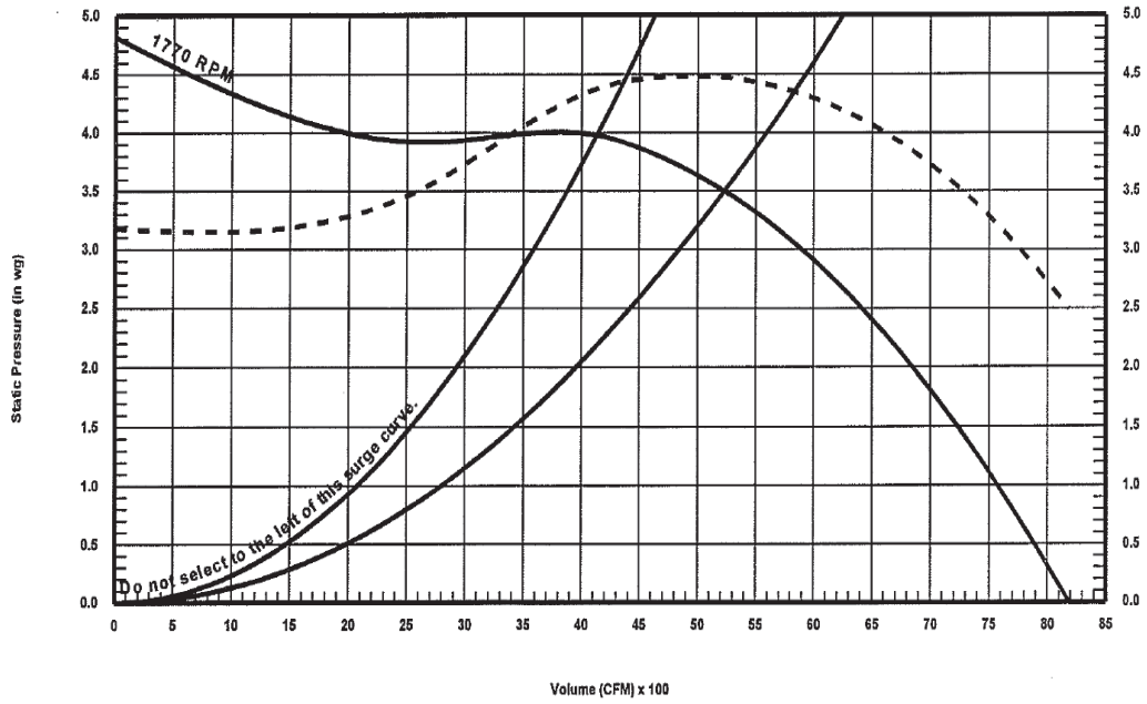
Figure 4. RSAU0010F0-F1 fan curve
