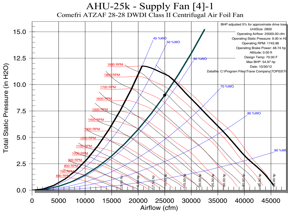
Figure 19. RSAU0062F1 fan curve
