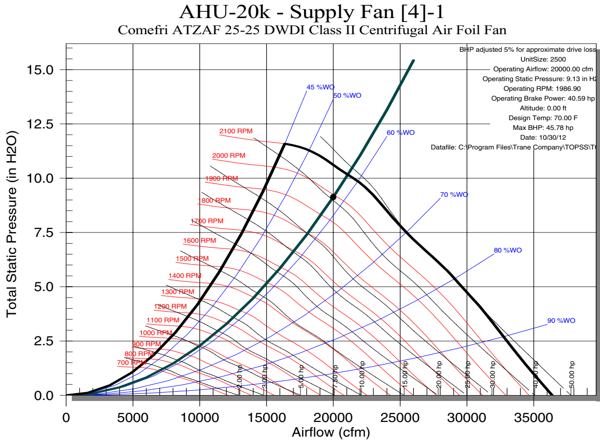
Figure 15. RSAU0050F1 fan curve
