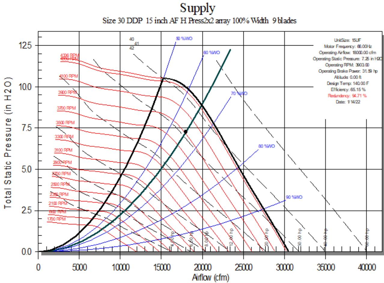
Figure 23. RSCC0030F0 supply fan curve
