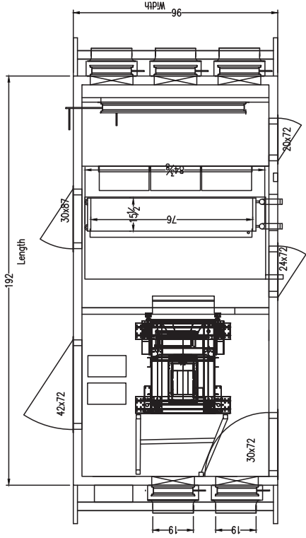
4 Plan View
