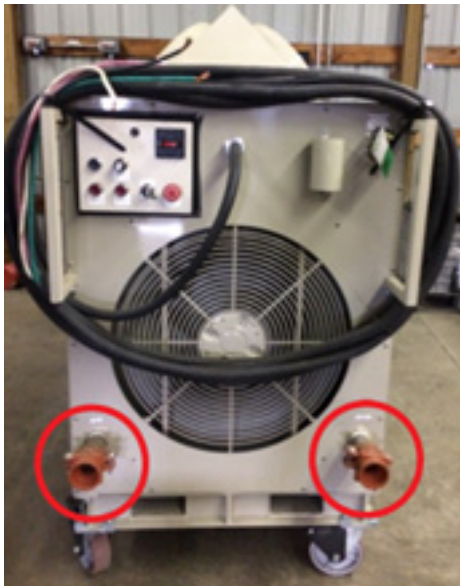
Figure 37. RSAU0010F1 - Victaulic water lines
