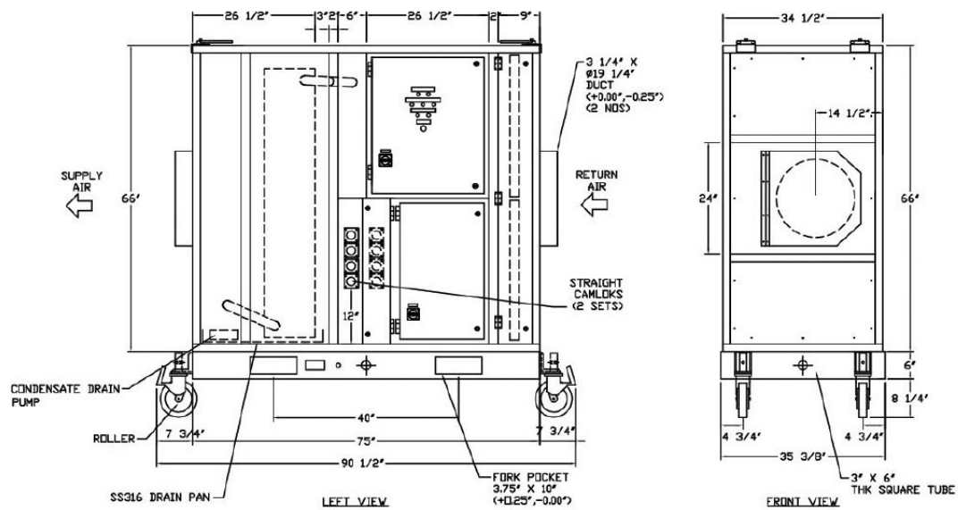
Figure 10. RSAU0010F2 unit drawing
