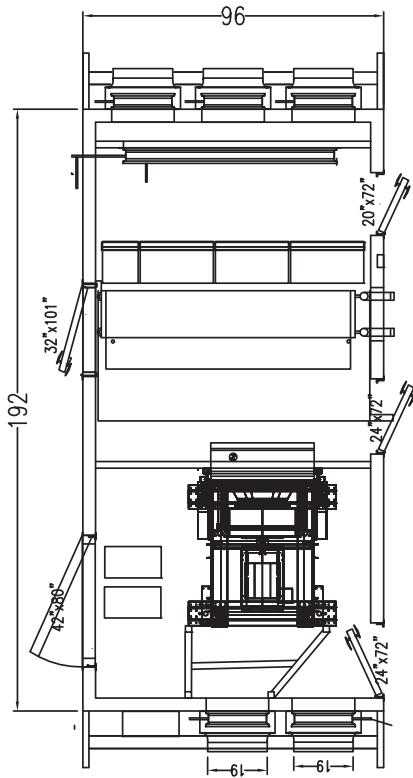
Plan View
