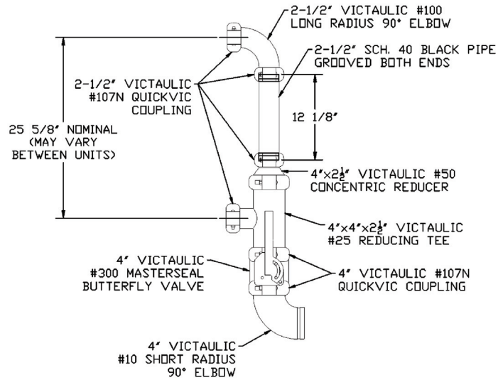
Figure 43. RSCC0030F0 - Manifold assembly
