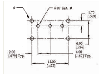
P.C. MOUNTING
