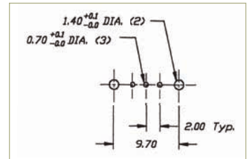
P.C. MOUNTING
