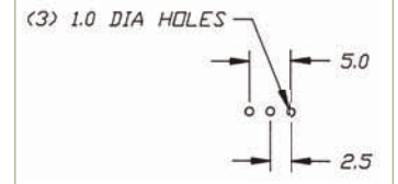
P.C. MOUNTING
