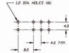
P.C. MOUNTING
