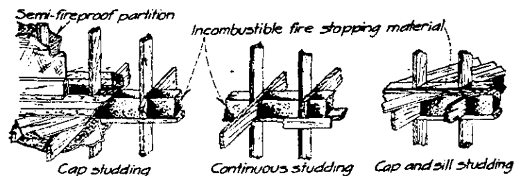
FIRE STOPPING
