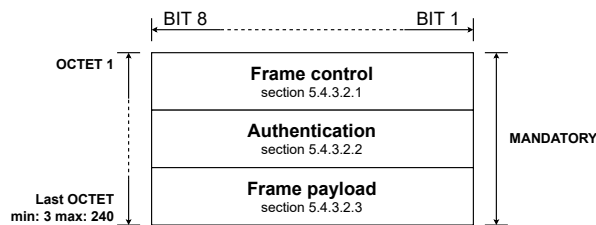
Fig. 5.14 Network layer - Blocks
