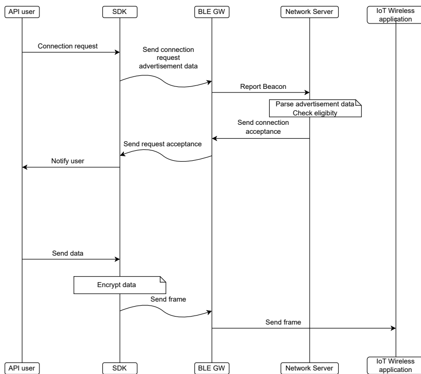
Fig. 6.17 BLE Endpoint initiated secure connection
