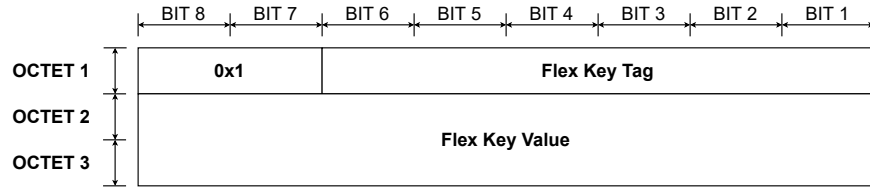
Fig. 6.15 Flex key coding - 2 bytes optimized format
