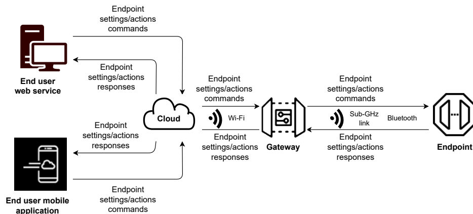
Fig. 2.3 End-user-interaction-with-an-endpoint
