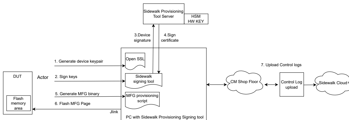
Fig. 4.7 Factory provisioning
