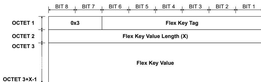
Fig. 6.13 Flex key coding - Standard format
