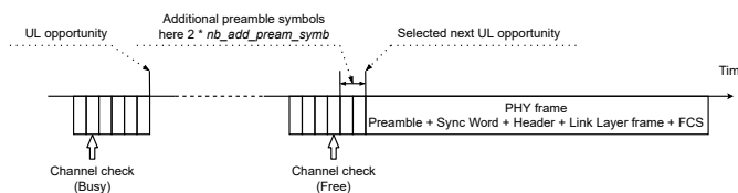
Fig. 5.57 SubG-FSK connection - Data transmission - Forbidden
