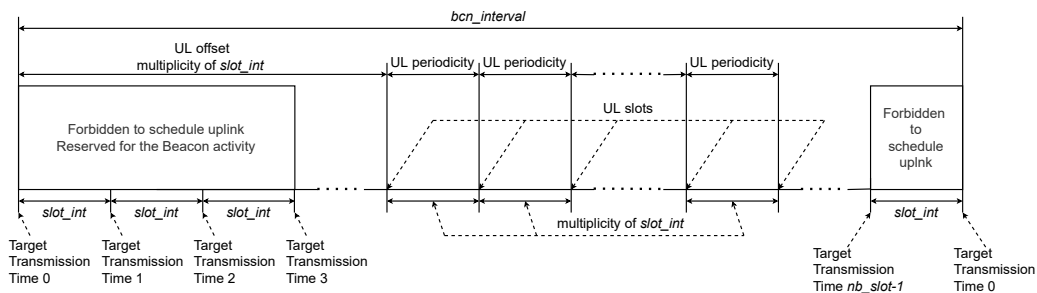
Fig. 5.51 SubG-FSK connection - UL scheduling
