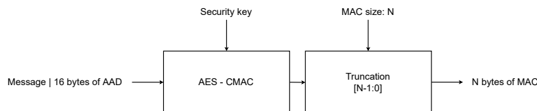
Fig. 4.17 MAC generation
