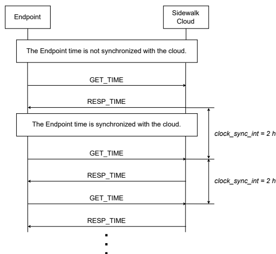
Fig. 7.2 Time sync maintenance
