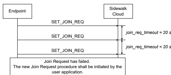
Fig. 7.4 Join Request no response
