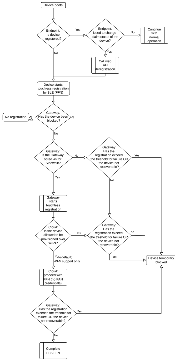
Fig. 6.19 BLE FFN touchless registration flow
