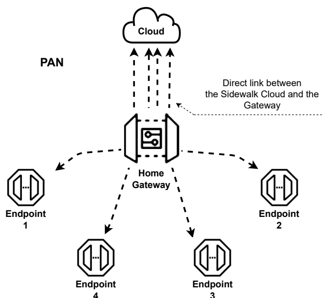
Fig. 2.4 Endpoint—cloud communication
