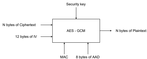
Fig. 4.14 Network layer security - packet decryption
