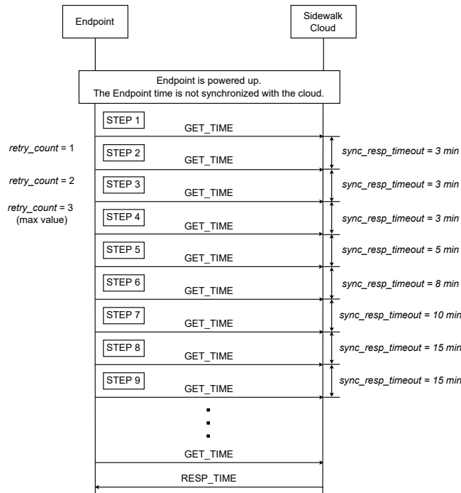
Fig. 7.3 Time sync - no response scenario
