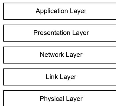
Fig. 5.1 Protocol stack
