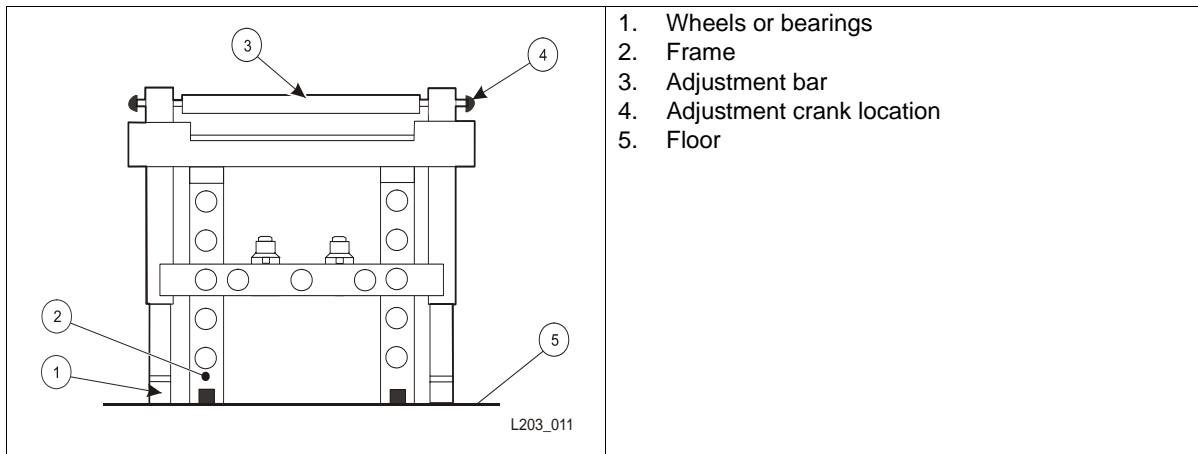
Figure 39. Adjustable Jack
