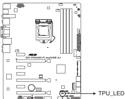
LED TPU de la Z97-PRO (Wi-Fi ac) / USB 3.1
