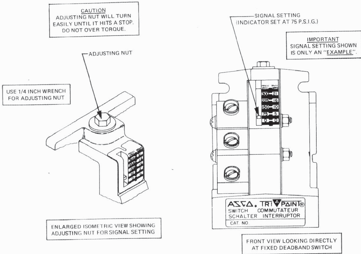
Adjustment (Signal Setting) of Fixed Deadband Switch
