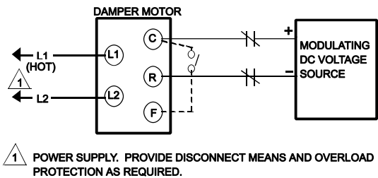
Fig. 6. Series 71 optional override switches to drive motor open or closed.
