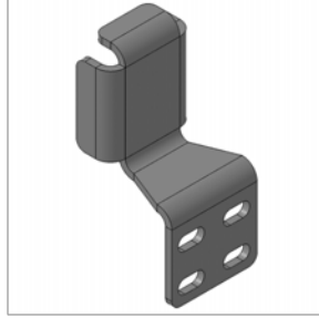
10044227 BRACKET,MTG,ATS,DPF,EPA15,T3RE
