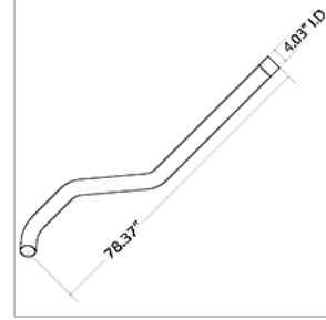
00119905 PIPE,EXH,STL,RR AXLE,PROPANE,FWD BBCV
