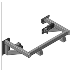
10044230 BRACKET ASSY,EXHAUST,DPF/SCR,EPA15,T3RE
