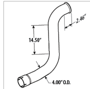
00056143 PIPE ASSY,EXHAUST,TURBO,CAT BBCV
