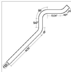
00000708 PIPE,EXHAUST,FRT AXLE CLEARANCE,4.0 OD HDPE
