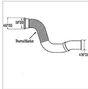
00118223 TUBE, EXHAUST, ENGINE TO MUFFLER, FWD, ISB
