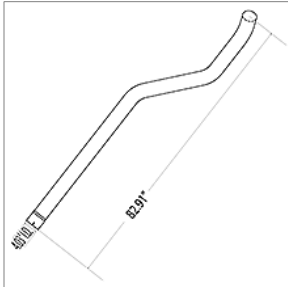
00000095 PIPE,EXH,RR AXLE CLER,FRT,SPR SUSP,4OD HDFE
