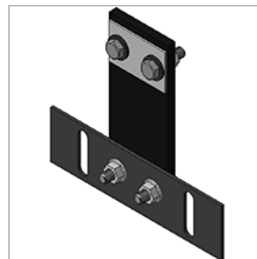
10040842 BRACKET ASSY,EXH,HANGER,ADJUSTABLE,6.50
