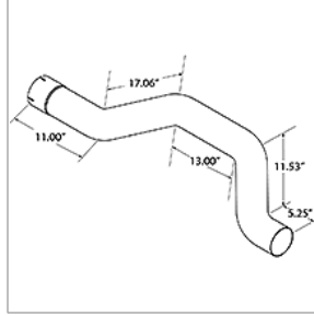
10011474 PIPE,EXH,SCR TO AXLE CLR, AIR SUSP,238WB
