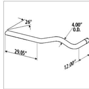
01997741 TAILPIPE, EXHAUST, LH SIDE EXHAUST, 4 OD HDFE
