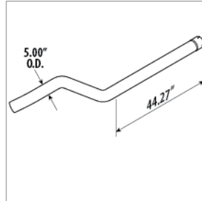
00003167 PIPE,EXH,RR AXLE CLER,FRT,SPR SUSP,5OD HDFE
