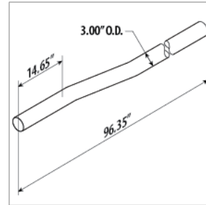
01622521 PIPE,EXH,FRT AXLE CLEARANCE,216-237WB TCFE
