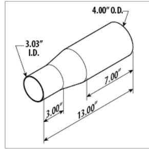
01375609 PIPE,EXHAUST,TRANSITION,3 ID TO 4 OD TCFC
