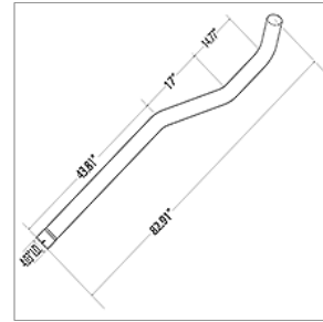
00000094 PIPE,EXH,RR AXLE CLER,FRT,AIR SUSP,4OD HDFE
