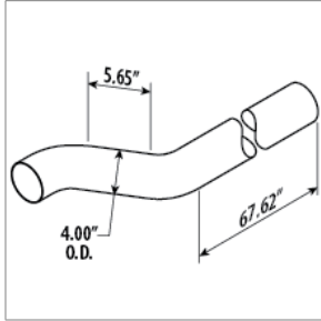
01493402 TAILPIPE, THRU BUMPER, 4.00 OD, 62.13 TCFC
