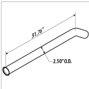
10018358 PIPE,EXHAUST,FLEX TO ELBOW,CAT C707,CV
