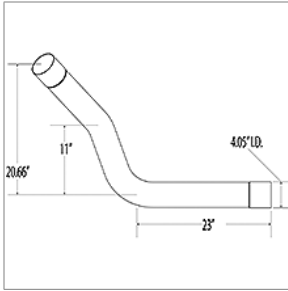
00119906 PIPE,EXH,STL,RR AXLE,PROPANE,REAR BBCV
