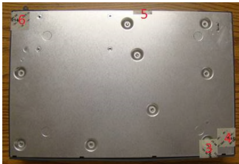
Figure 26 - Required TELs for the Aruba 7205 Mobility Controller – Bottom
