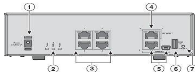
Figure 4 ASA 5506H-X Appliance Rear Panel
