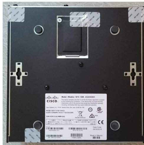
Figure 30 ASA 5506H-X Bottom TEL Placement
