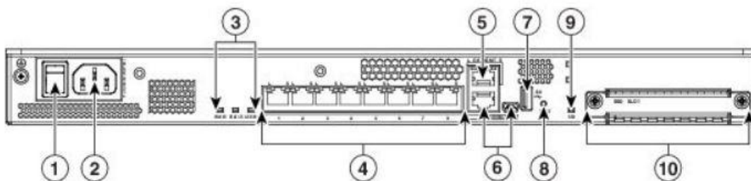
Figure 6 ASA 5508-X and ASA 5516-X Appliances Rear Panel
