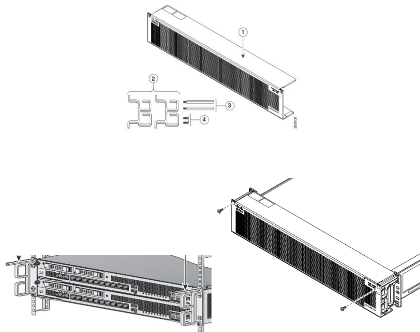
Figure 18 ASA 5585-X Opacity Shield Placement
