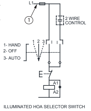
ILLUMINATED HOA SELECTOR SWITCH
