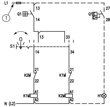
Maintained Control, Selector Switch < O >
