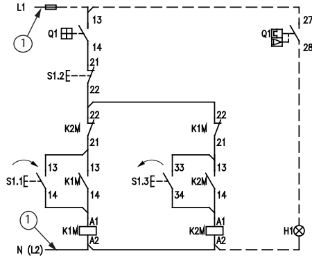
Impulse Control, Multi Function Push Button ① L1 control voltage supplied from external source.
