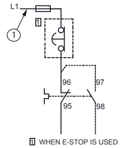
ILLUMINATED HOA SELECTOR SWITCH
