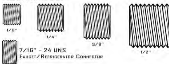
MALE NPT FITTING SIZES
