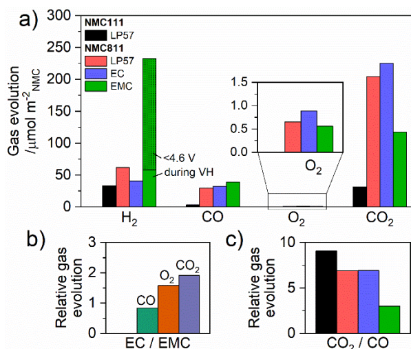
Figure 3. (a) Quantity of \text{H}_2 , CO, \text{O}_2 , and \text{CO}_2 gases evolved in the OEMS experiments shown in Figure 2. The inset shows a magnified view of \text{O}_2 . (b) Fraction of CO, \text{O}_2 , and \text{CO}_2 evolved with NMC811 and 1.5 M \text{LiPF}_6 in ethylene carbonate (EC) electrolyte relative to 1.5 M \text{LiPF}_6 in ethyl methyl carbonate (EMC) electrolyte (EC/EMC). (c) Fraction of \text{CO}_2 relative to CO ( \text{CO}_2/\text{CO} ) for each NMC-electrolyte pairing.
