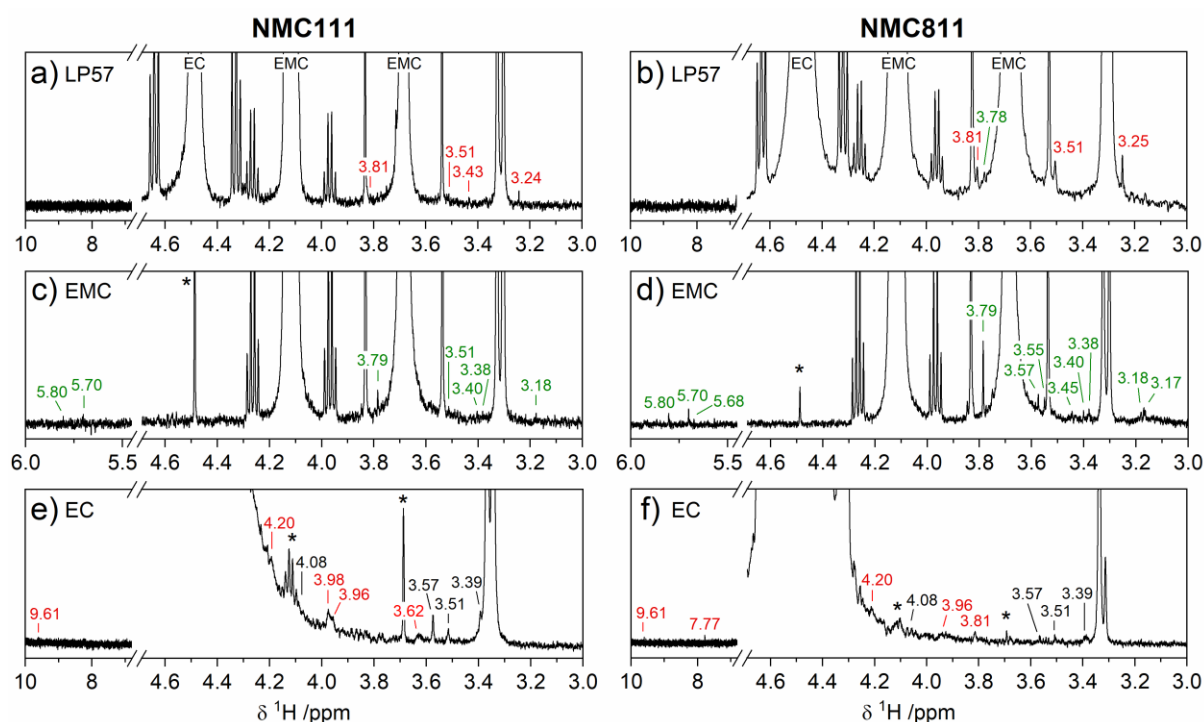
Figure 7. ^1\text{H} NMR spectra of the electrolyte extracted from NMC/LTO cells after the first charge-discharge cycle between 1.45-3.05 V at C/20 with a 60 h potentiostatic hold at 3.05 V for (left; a, c, e) NMC111 and (right; b, d, f) NMC811 with electrolytes (a-b) LP57, (c-d) 1.5 M \text{LiPF}_6 in ethyl methyl carbonate (EMC), and (e-f) 1.5 M \text{LiPF}_6 in ethylene carbonate (EC). Signals of EC and EMC are annotated in (a) and (b). Signals of a trace EC impurity in 1.5 M \text{LiPF}_6 in EMC electrolyte, and a trace EMC impurity in 1.5 M \text{LiPF}_6 in EC electrolyte, are marked in (c-f) with an asterisk. The chemical shift labels in black are also present in the pristine electrolyte, while green and red correspond to signals that arise from EMC and EC degradation, respectively.
