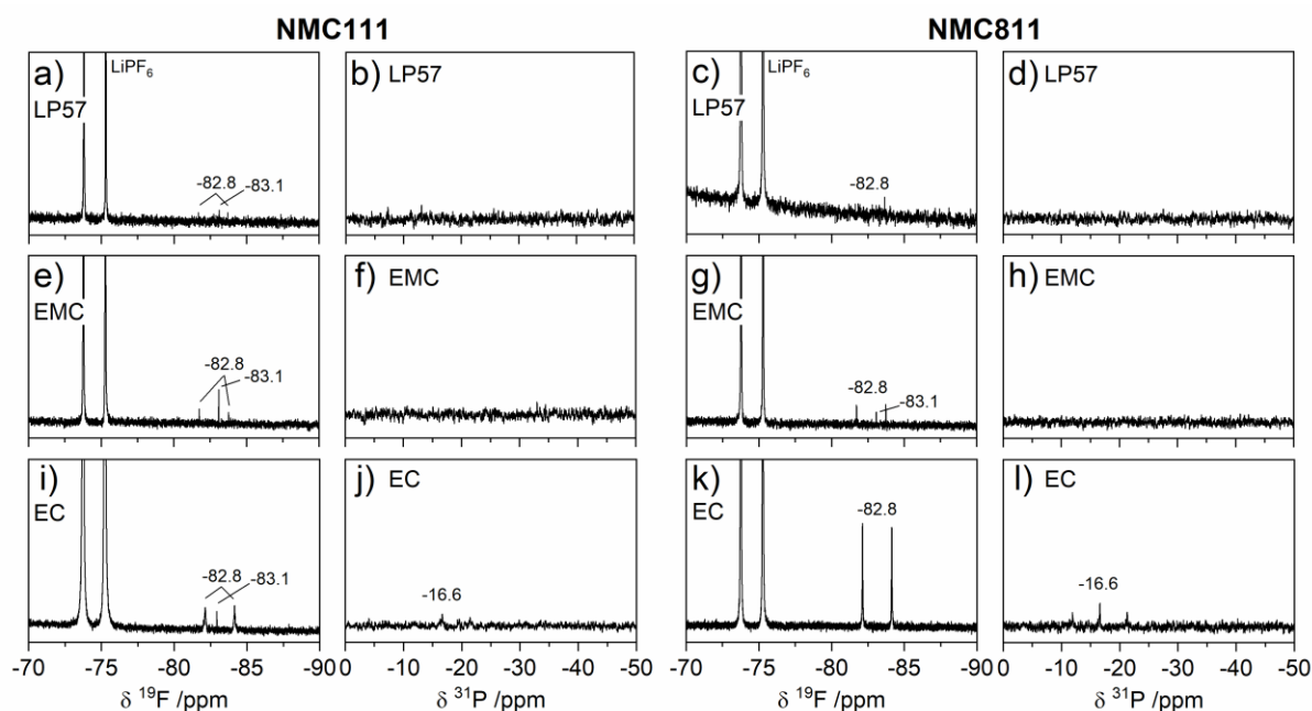
Figure 8. ^{19}\text{F} and ^{31}\text{P} NMR spectra of the electrolyte extracted from NMC/LTO cells after the first charge-discharge cycle between 1.45-3.05 V at C/20 with a 60 h potentiostatic hold at 3.05 V for (left; a-b, e-f, i-j) NMC111 and (right; c-d, g-h, k-l) NMC811 with electrolytes (a-d) LP57, (e-h) 1.5 M \text{LiPF}_6 in ethyl methyl carbonate (EMC), and (i-l) 1.5 M \text{LiPF}_6 in ethylene carbonate (EC). Signals of \text{PF}_6^- are annotated in (a) and (c).
