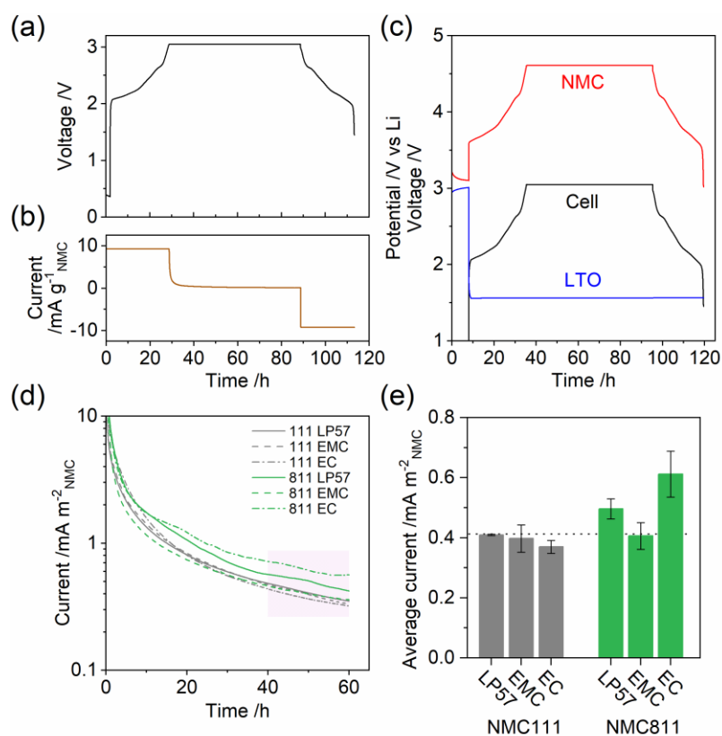
Figure 1. Representative (a) voltage and (b) current profiles for a NMC/LTO coin cell during the first charge-discharge cycle between 1.45-3.05 V at C/20 with a 60 h potentiostatic hold at 3.05 V. Data is shown for NMC811/LTO with LP57 electrolyte. (c) Potential profiles of the NMC811 cathode and LTO anode in a three-electrode cell with a Li metal reference
