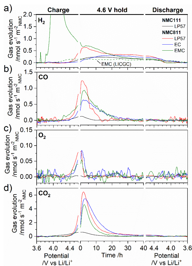
Figure 2. Evolution of (a) \text{H}_2 , (b) \text{CO} , (c) \text{O}_2 , and (d) \text{CO}_2 as determined from the OEMS channels m/z = 2, 28, 32, and 44 , respectively, and normalized to the NMC surface area. For NMC/Li cells during the first charge-discharge cycle between 2.5-4.6 V at C/20 with a 40 h potentiostatic hold at 4.6 V. For NMC111 with LP57 electrolyte and NMC811 with electrolytes LP57, 1.5 M \text{LiPF}_6 in ethyl methyl carbonate (EMC), and 1.5 M \text{LiPF}_6 in ethylene carbonate (EC). Data are plotted as a function of potential for the charge and discharge, and time for the potentiostatic hold. The evolution of \text{H}_2 for a NMC811/Li cell with a lithium ion conducting
