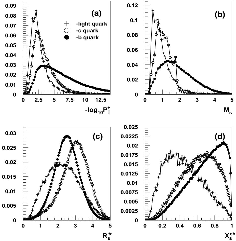
Figure 4.25: Distributions of discriminating variables used in the combined impact parameter tagging: (a) the jet lifetime probability, \mathcal{P}_j^+ ; (b) the effective mass distribution of particles included in the secondary vertex, M_s ; (c) the rapidity distribution of tracks included in the secondary vertex with respect to the jet direction, R_s^{tr} ; (d) the fraction of the charged energy distribution of a jet included in the secondary vertex, X_s^{ch} .
