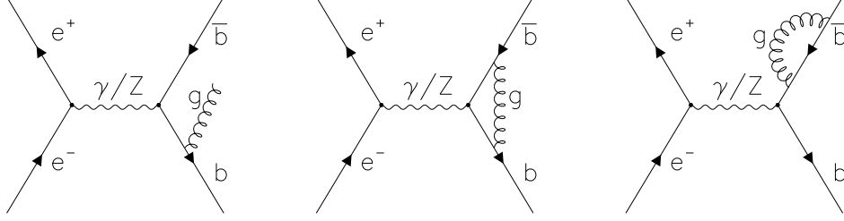
Figure 2.4: Examples of QCD radiative processes in e^+e^- \rightarrow \text{hadrons} .
