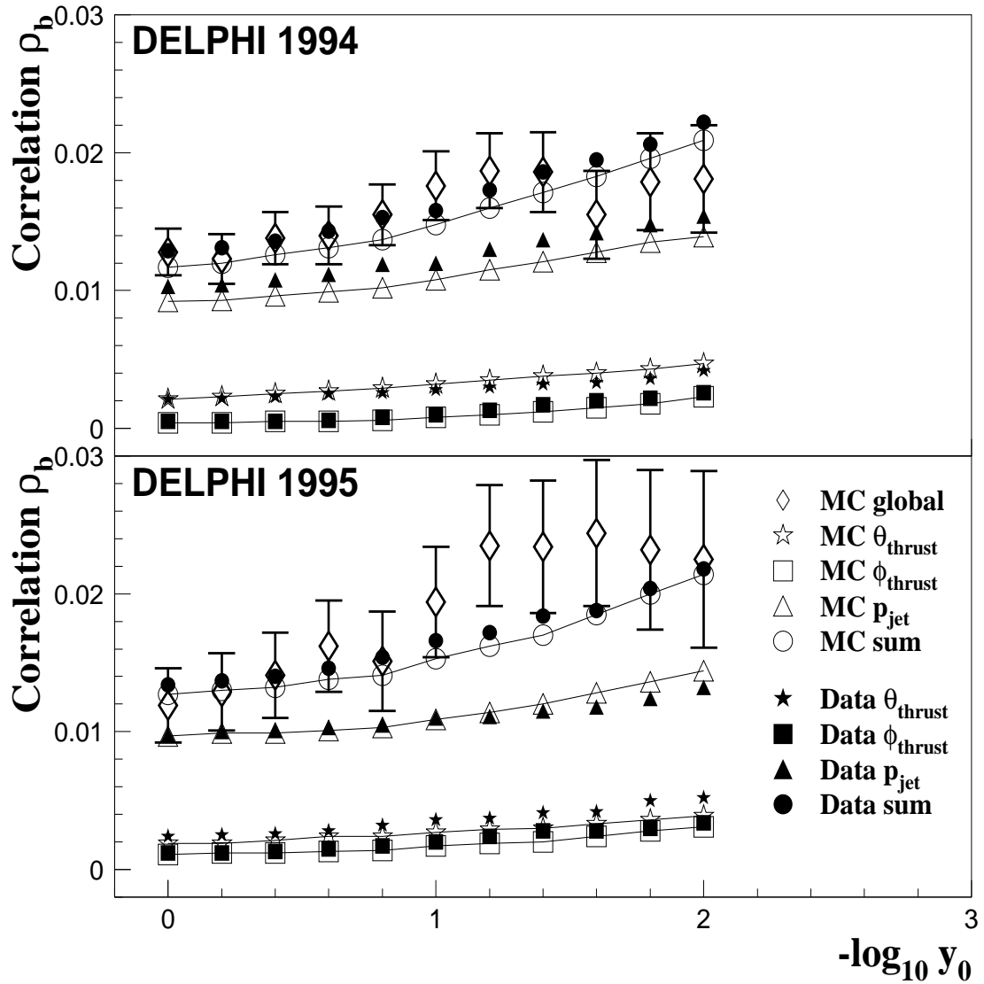
Figure 6.7: Global correlation ( \rho_b or \rho_{b\text{-tight},b\text{-tight}}^b ) for the b-tight tag as a function of the cut value -\log_{10} y_0 for the 1994 and 1995 analyses, together with each of the three main correlation components and their sum, for data and simulation. Points are bin-to-bin correlated.
