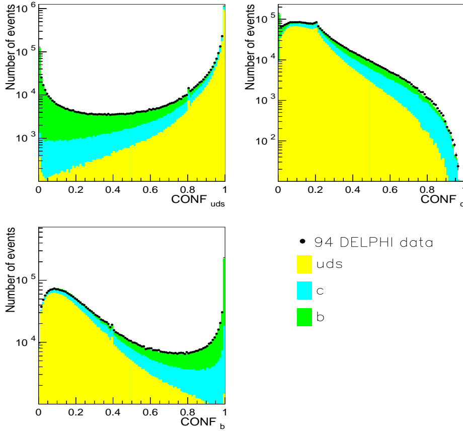
Figure 4.17: Distribution of uds, c and b confidences in 1994 simulation and data. Real data are superimposed to show the quality of the Monte Carlo description of the data. The contribution of uds, c and b flavour is also shown for the simulation.
