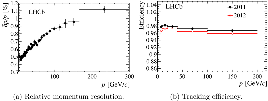
Figure 3.13 – Relative momentum resolution for long tracks (a) and tracking efficiency (b) as a function of the momentum.
