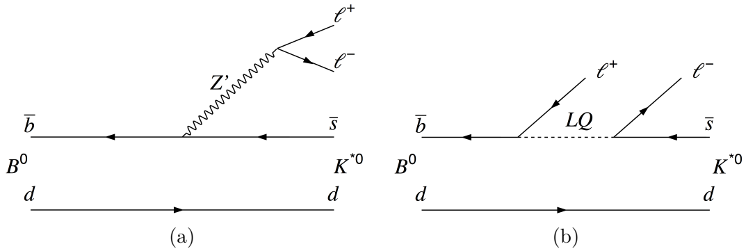
Figure 2.2 – Potential New Physics diagrams, with an additional Z' boson (a) and a Leptoquark (b) for the B^0 \rightarrow K^{*0}l^+\ell^- decay.
