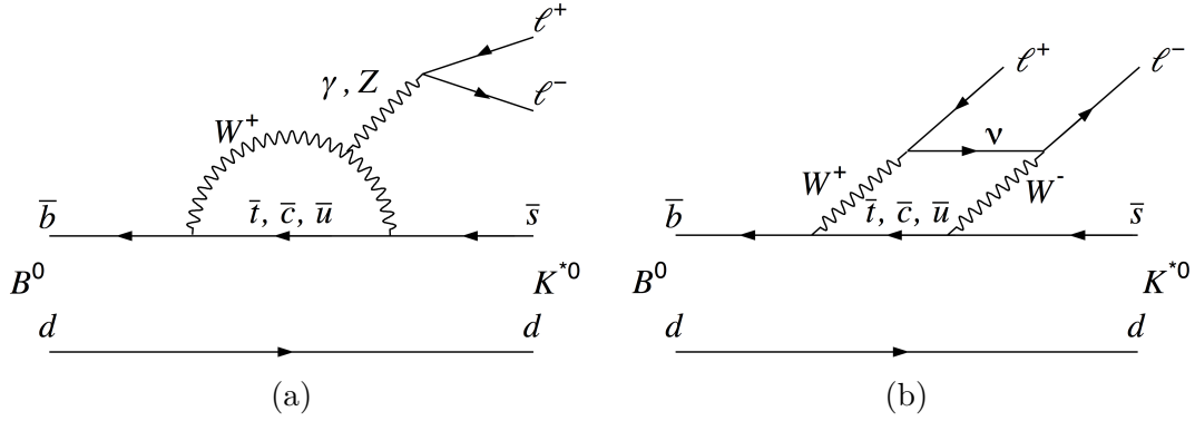
Figure 2.1 – Standard Model penguin (a) and box (b) diagrams for the B^0 \rightarrow K^{*0}l^+\ell^- decay.
