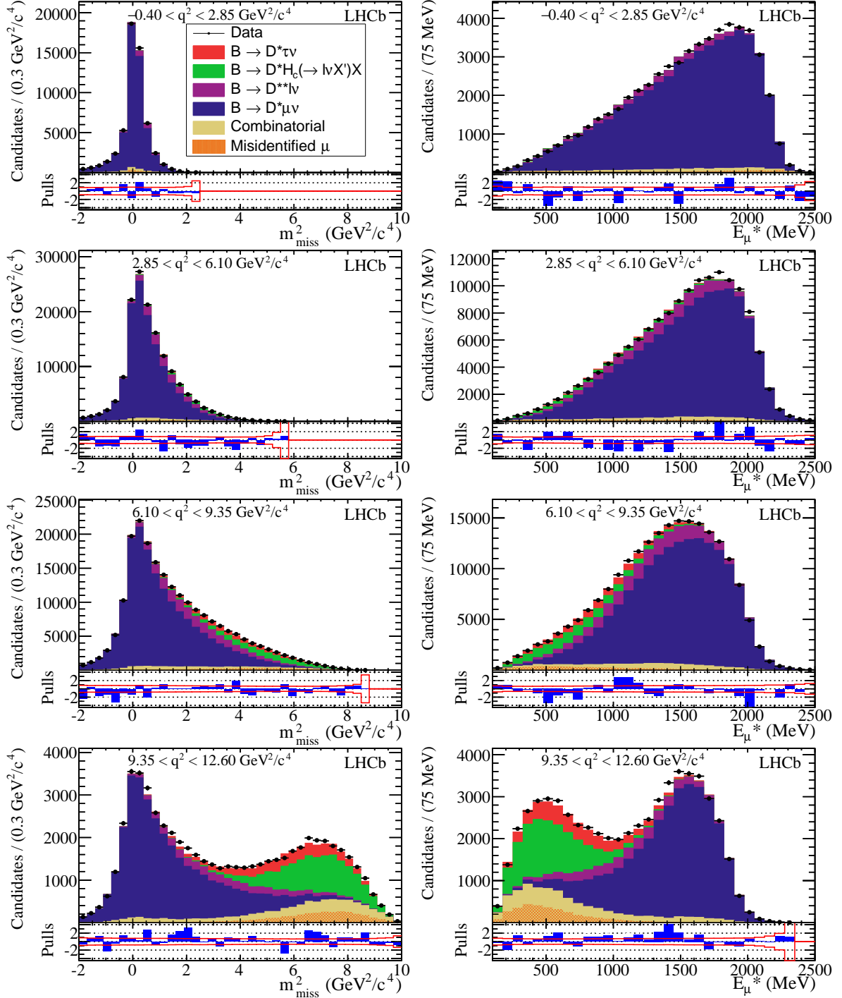
Figure 2.6 – Fit results as a function of m_{miss}^2 and E_{\mu}^* in bins of q^2 . Figure taken from Ref. [67].
