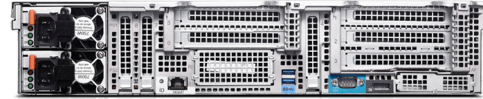
ThinkServer RD650 - Rear view (All chassis types share one rear view)
