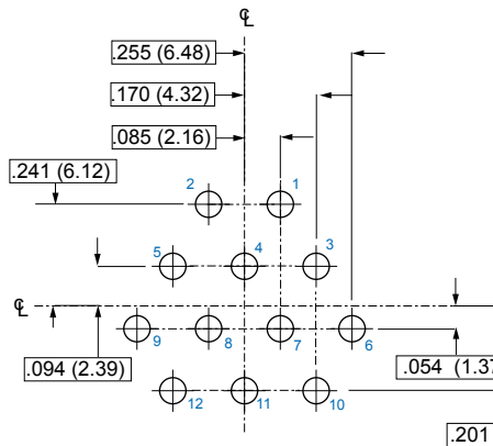
Insert Arrangement 14-12, 16-12, 18-12 12 #16 Contacts .064 (1.63) Max Dia. Tail
