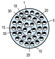
Insert Arrangement 14-235, 16-235, 18-235 35 #20HD Contacts .028 (0.71) Max. Dia. Tail
