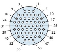
Insert Arrangement 14-55, 16-55, 18-55 55 #23 Contacts .022 (0.56) Max. Dia. Tail
