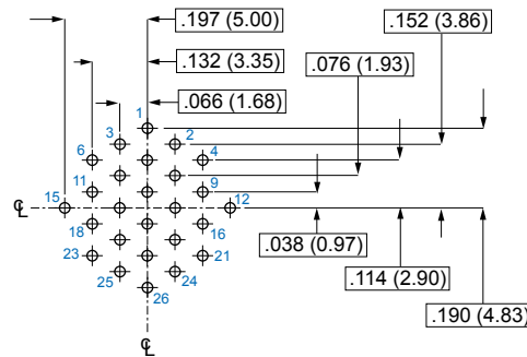
Insert Arrangement 10-26, 12-26 26 #23 Contacts .022 (0.56) Max. Dia. Tail
