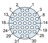
Insert Arrangement 11-31, 13-31 26 #23 Contacts .022 (0.56) Max. Dia. Tail
