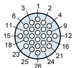
Insert Arrangement 10-26, 12-26 26 #23 Contacts .022 (0.56) Max. Dia. Tail
