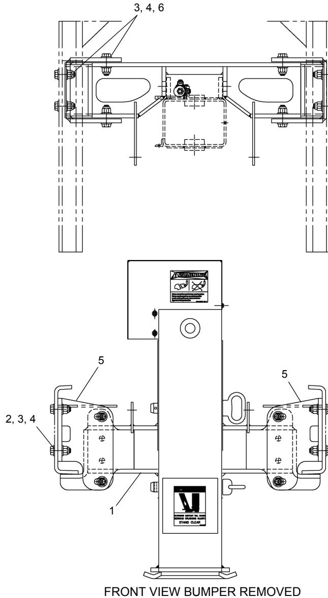
FRONT VIEW BUMPER REMOVED
