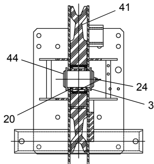
SECTION K-K
