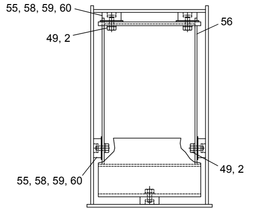
SECTION J-J
