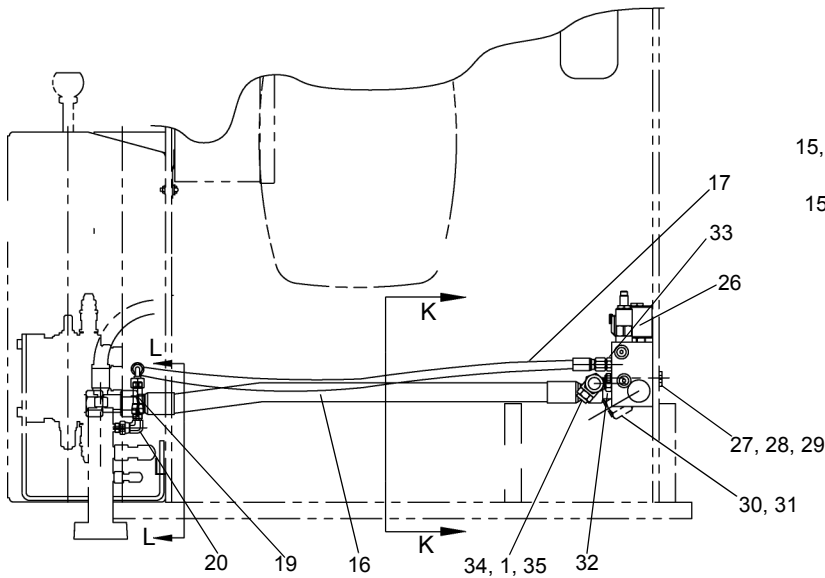
VIEW H - H GREER BOX
