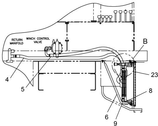
CURBSIDE INSTALLATION
