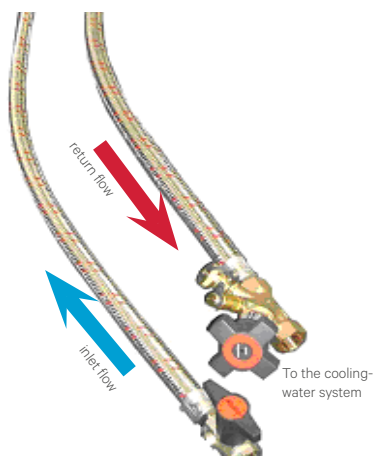
Draining and purging valve with nipple for measurement device connection (3/4", female) (for measuring water flow rate)
