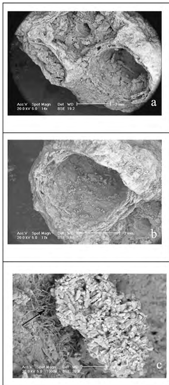
Figure 10. SEM images of cave crystals collected from the speleothem in Grave Grubbo Cave. a ) Cross-section of the aggregate showing the outer-inner laminae and the middle, sponge-like septa. b ) Detail of a . c , Spike crystals deposited after tube formation are likely to occlude the lumen of the tube. Filamentous calcified bacteria interacting with the calcite layer (arrow).
