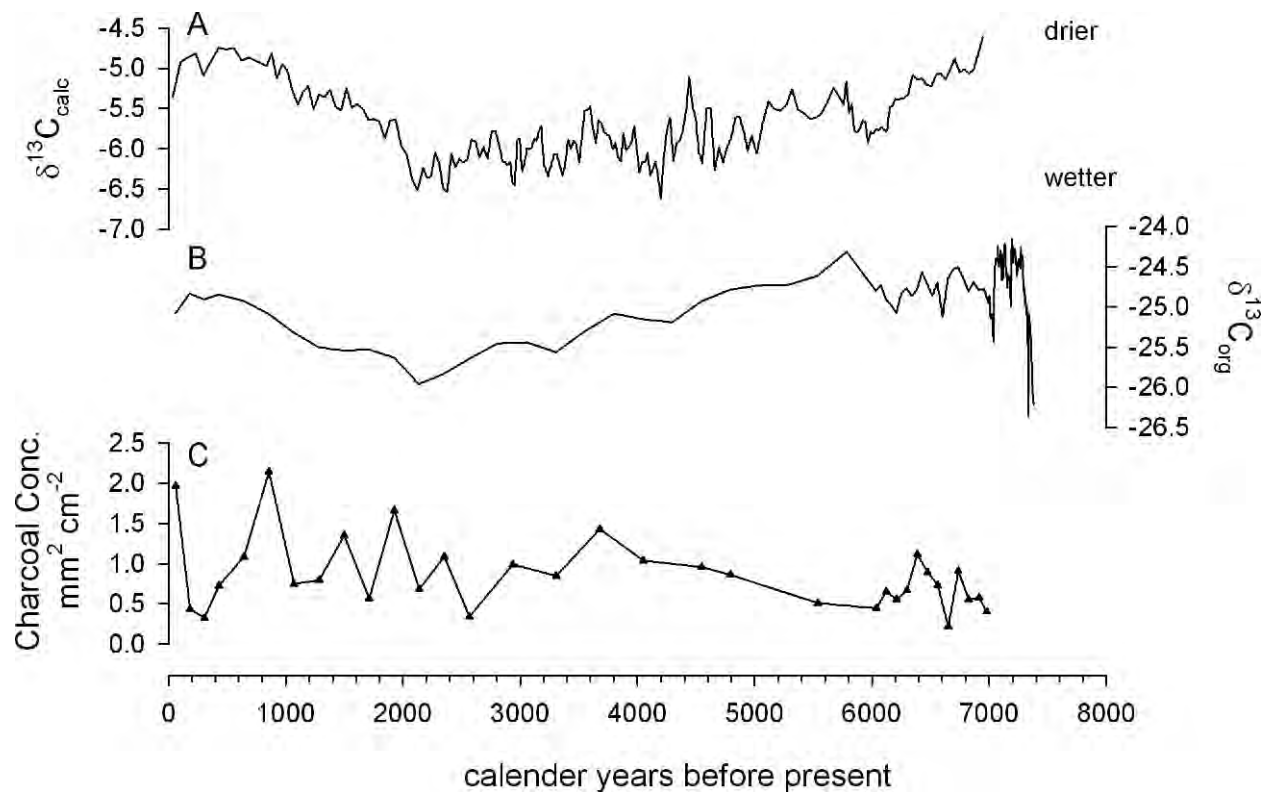
Figure 3. (A) A stable isotopic ( ^{13}\text{C}_{\text{calc}} ) paleoclimatic record obtained from a stalagmite records long-term changes in the soils and ecosystem above Buckeye Creek Cave (Springer et al., 2008). Moisture levels increased from the mid to late Holocene, but ^{13}\text{C}_{\text{calc}} values increased abruptly \sim 100 BC. This coincides with use of Unnamed Cave #14 (UC14) by Native Americans, and values peak approximately when Native Americans were making their most extensive use of UC14 (Maslowski, 2006). Other regional paleoclimatic records do not record drying after 2,100 years BP (Springer et al., 2009; 2010), but the anomalous ^{13}\text{C}_{\text{calc}} record is corroborated by stable isotopic analysis of organic material ( ^{13}\text{C}_{\text{org}} ) in the Trench Five sediments (B). (C) Fire activity was high during the Late Holocene and peaks near the times of peak ^{13}\text{C}_{\text{calc}} and ^{13}\text{C}_{\text{org}} values, coinciding with peak Native American use of the watershed, as inferred from the UC14 record (McBride and Sherwood, 2006).
