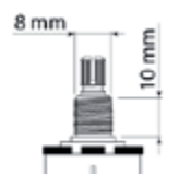
500K potentiometer, 10mm. bushing, M8x0,75 thread, made in Taiwan 31836 ALP500-A43 audio 31837 ALP500-B44 linear
