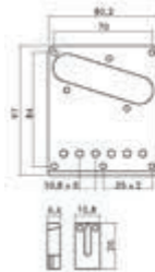
bridge-tailpiece, Teaser, block saddles, flat plate
