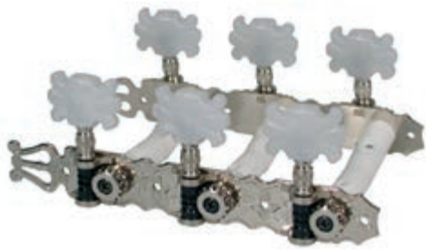
machine heads for classic guitar, nylon shaft, 3x left+3x right, 70mm, nickel
