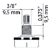
500K potentiometer, standard length bushing .375", 3/8" diameter, made in Taiwan 31827 ALP500-A33 audio 31828 ALP500-B34 linear
