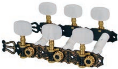
machine heads for classic guitar, nylon shaft, 3x left+3x right, 70mm, black engraved
