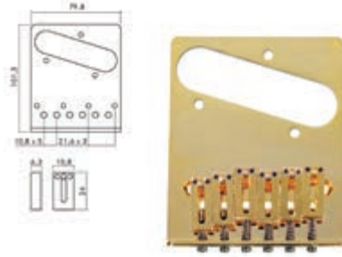
bridge-tailpiece, Teaser, gold, block saddles, flat plate
