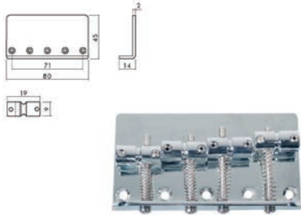
bridge-tailpiece, Jocker/ Puncher bass, pitch 19mm
