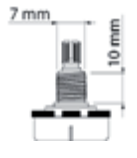
2x500K blender potentiometer, 10mm. bushing, M7x0,75 thread, blends 2 sources, made in Japan 14111 PM-500-Z
