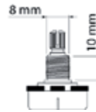
250K potentiometers, 6 pcs, 10mm. bushing, M8x0,75 thread, made in Korea 21468 PM-1250-B linear (tone) 21469 PM-1250-A audio (volume)
