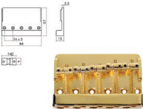
bridge-tailpiece, Jocker/ Puncher bass, 5-string, pitch 16mm 16794 BB-505-G gold
