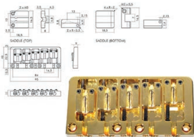
bridge-tailpiece, WMI-model, 5-string, pitch 16,5mm 16809 BB-705-G gold
