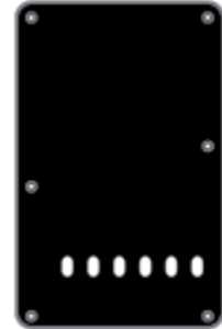
back plate, string spacing 11,2mm, 4 ply, standard Stallion, 86x138mm 32654 BP-413-PB pearl black
