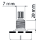
kill pot potentiometer, machine gun effect, 250K, long bushing, M7x0,75 thread 32946 SH-124-250
