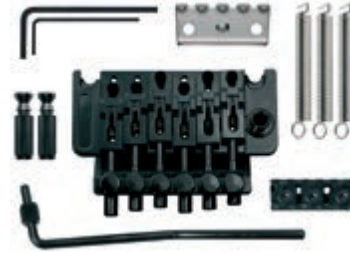
tremolo "Floyd Rose", single lock 23406 TFR-225-C chrome 23407 TFR-225-B black 23408 TFR-225-G goldplated
