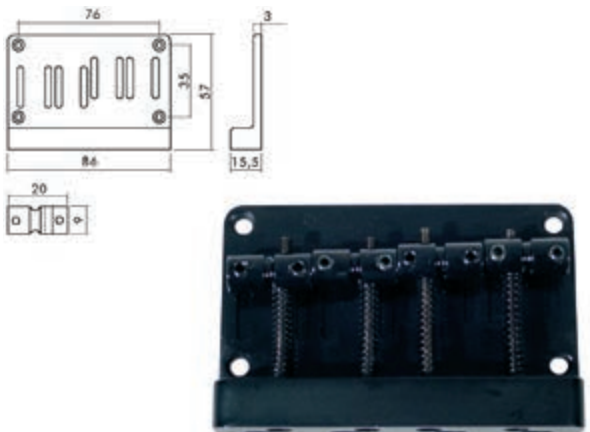
bridge-tailpiece, Jocker/ Puncher bass, pitch 20mm
