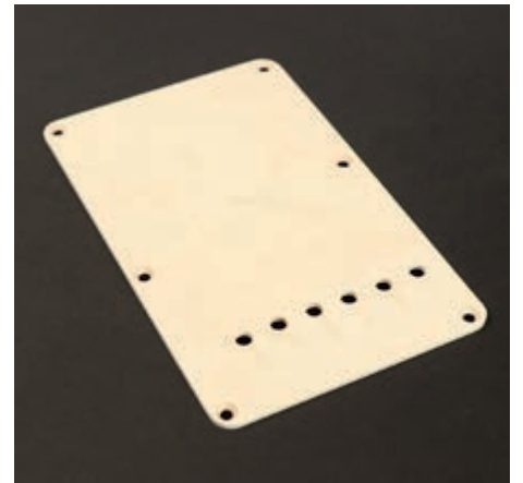
Master Relic Series back plate, string spacing 11,2mm, 1 ply 42763 BP-105RE white relic
