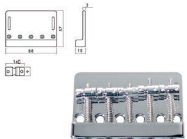
bridge-tailpiece, Jocker/ Puncher bass, 5-string, pitch 16mm
