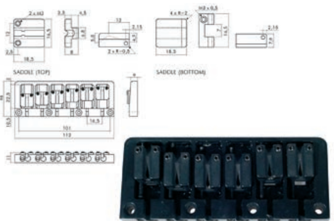
bridge-tailpiece, WMI-model, 6-string, pitch 16,5mm 16811 BB-706-B black 16812 BB-706-G gold
