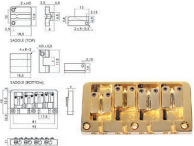
bridge-tailpiece, WMI-model, pitch 20mm 16806 BB-704-G gold
