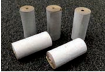
self-adhesive sandpaper suitable to use with H-SB sanding blocks 42799 KCR100 100 grit, 1,4m 42800 KCR120 120 grit, 1,8m 42801 KCR150 150 grit, 2,2m 42802 KCR240 240 grit, 2,6m 42803 KCR320 320 grit, 3,2m 42804 KCR400 400 grit, 3,2m 42805 KCR600 600 grit, 3,2m
