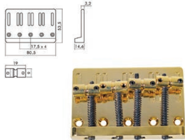
bridge-tailpiece, Jocker/ Puncher bass, pitch 20mm
