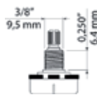
500K potentiometer, solid shaft, short bushing .250", 3/8" diameter, for pickguard 31831 ALP500-A37 audio 31832 ALP500-B38 linear
