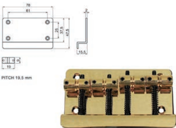
bridge-tailpiece, Jocker/ Puncher bass, pitch 20mm 27241 BB-123-G gold
