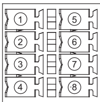
Front view of connector on controller side
