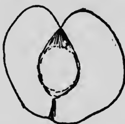
Fig. 21. Cardiocarpon Baileyi , Dawson. Outline tracing of original and only specimen of fig. 48, plate XIX.
