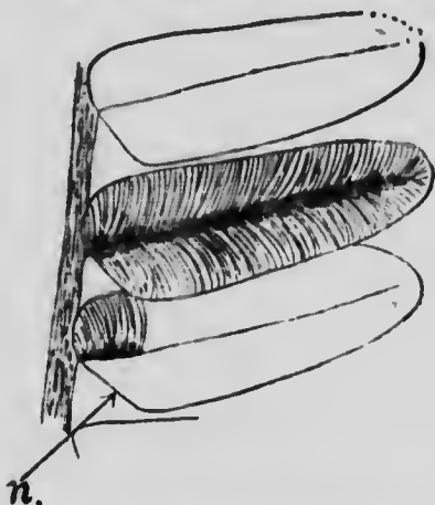
Fig. 12. Neuropteris belwyni , Dawson. Enlargement of the three central pinnules of Dawson's type specimen, to show their shape, veins and the "notch" n on the lower side of the pinnules. Original of Dawson's fig. 198; cf. fig. 37, pl. XV.
