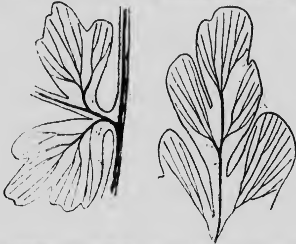
Fig. 2. Sphenoptera valida , Dawson, sp. Outline of terminal and basal pinnules to show shape and venation. Enlarged.
