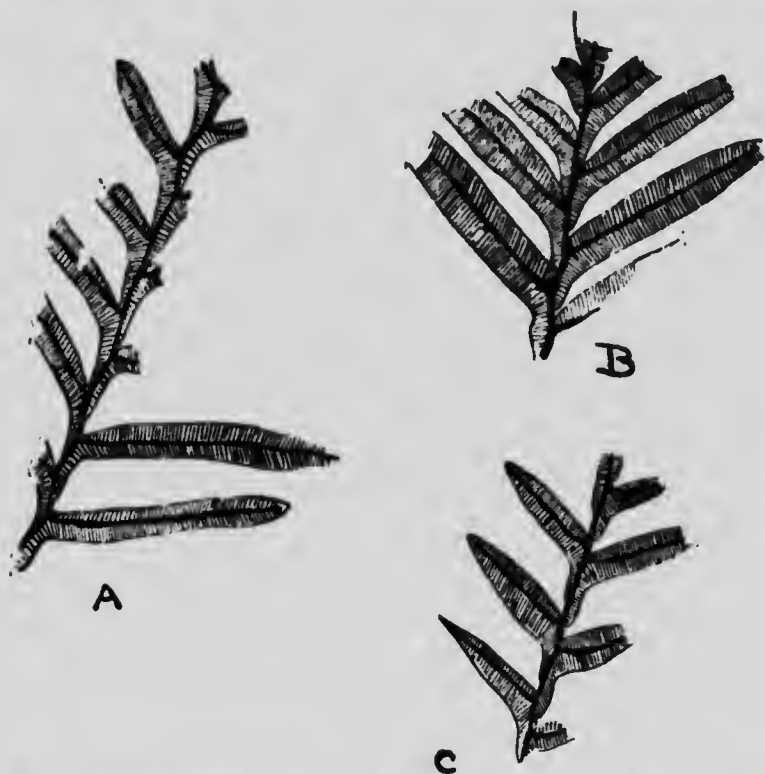
Fig. 8. Alethopteris lonchitica , Schlotheim, sp. A, tracing from Dawson's specimen of "A. discrepans" (fig. 30, pl. XII); B, tracing of Alethopteris lonchitica in Renier's pl. XCII; C, Alethopteris lonchitica from specimen 1 found at Joggins, Nova Scotia. In each case the asymmetrically placed midrib is evident, and the "discontinuous" decurrent bases of the pinnules.
