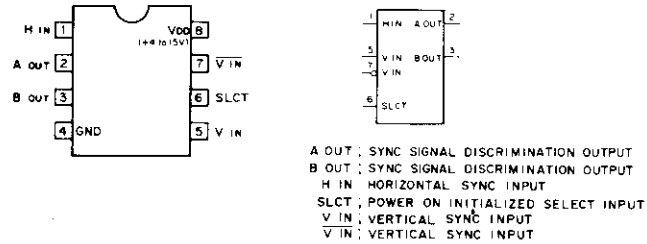
CX23025 (SONY) C-MOS TV-VTR SYNC SIGNAL DISCRIMINATOR — TOP VIEW —
