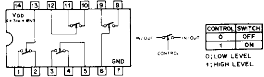
MC14066BCP C-MOS BILATERAL ANALOG SWITCH - TOP VIEW -
