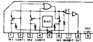
CX894 (SONY) 3 INPUT SWITCH — SIDE VIEW —
