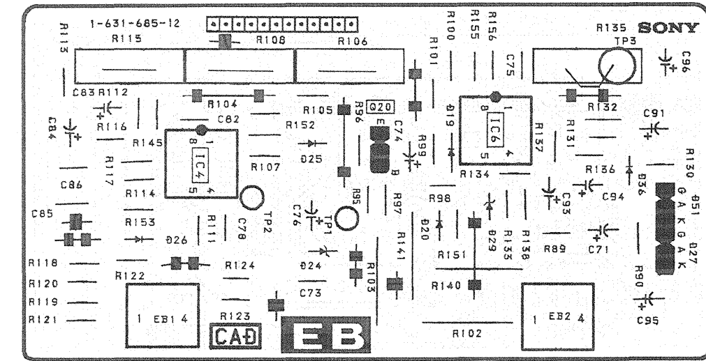
EB board (H.V, BEAM CURRENT & CRT PROTECTOR)
