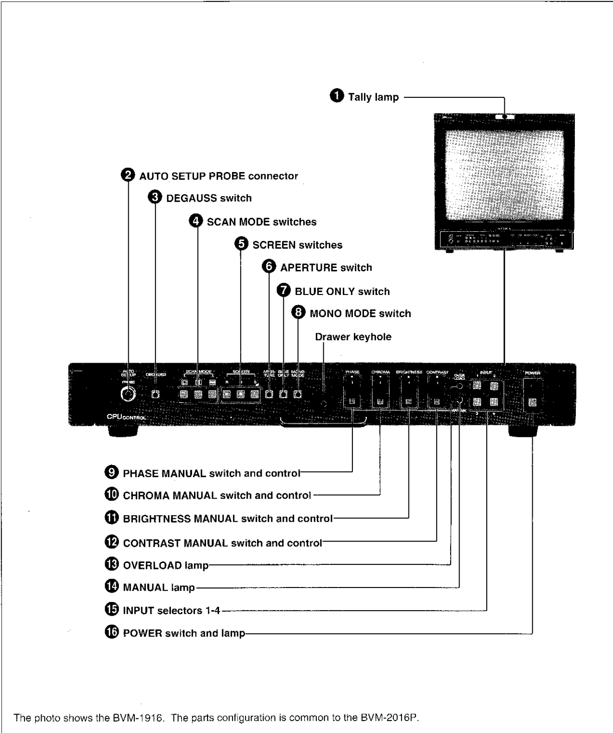
Front panel
