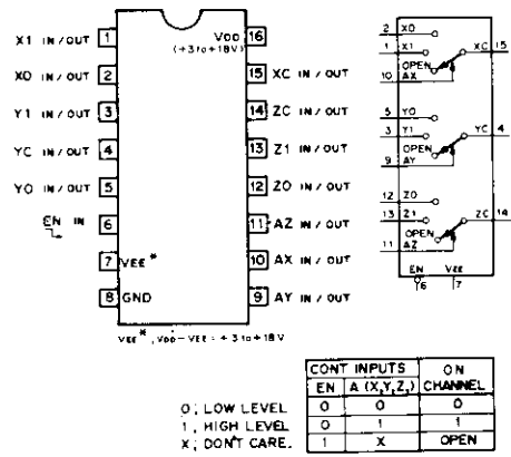
MC14053BCP (MOTOROLA) TC4053BP TC4053BPHB (TOSHIBA) μPC4053BC C-MOS 2-CHANNEL MULTIPLEXER/DEMULTIPLEXER - TOP VIEW -
