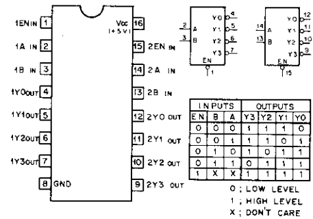
TC74HCT139AF TTL 2-TO-4-LINE DECODER/DEMULTEPLEXER - TOP VIEW -
