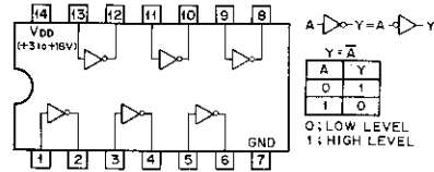
TC4069BP (TOSHIBA) CMOS INVERTER - TOP VIEW -
