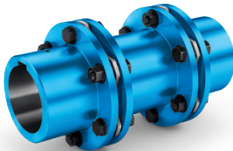
N-ARPEX and ARPEX all-steel couplings Rated torque: 92 Nm ... 2,000,000 Nm
