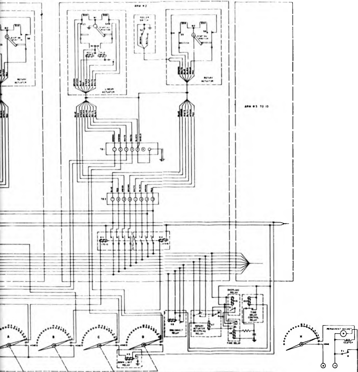
10 Schematic, Shallow Soil Sampler
