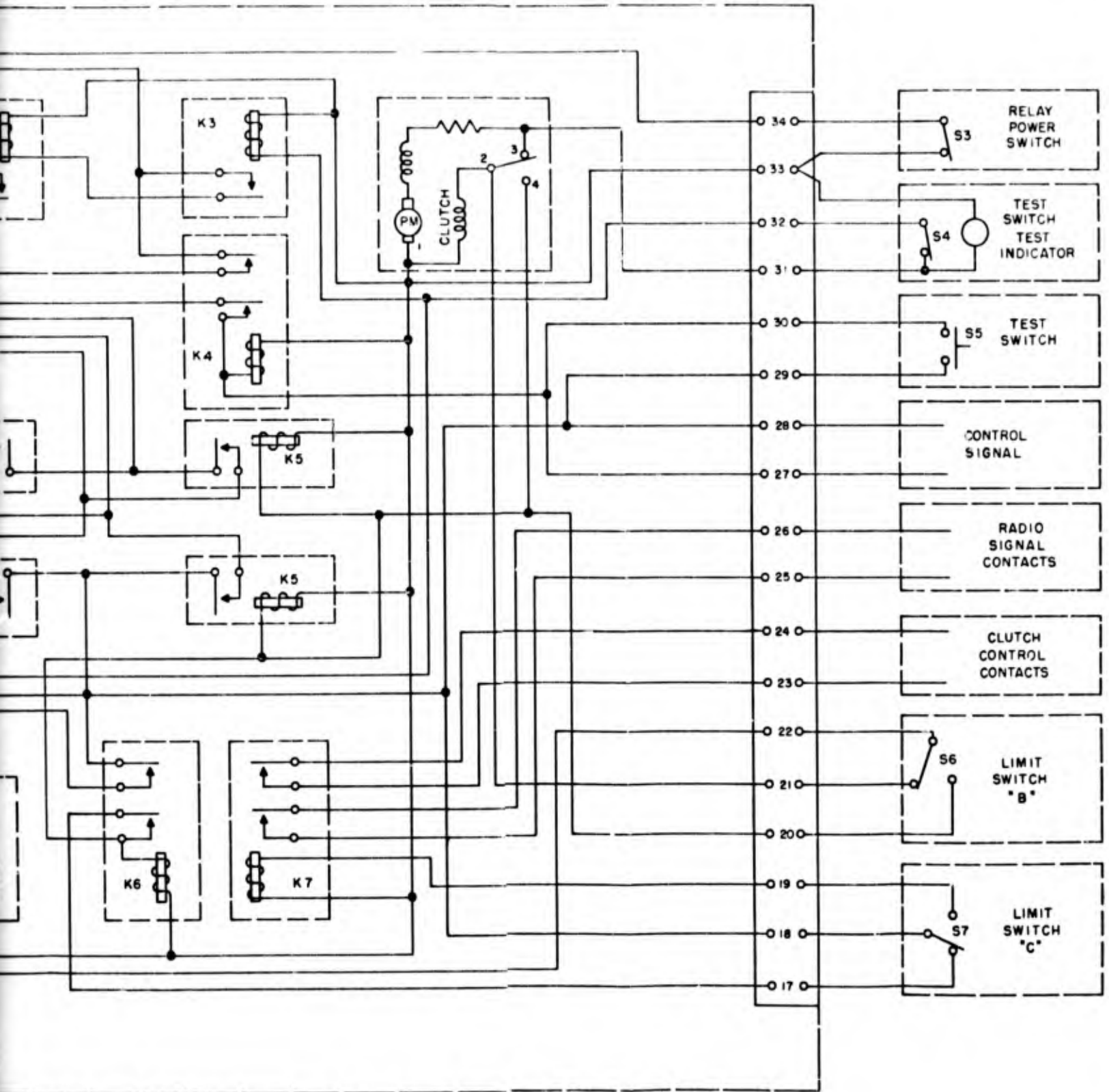
Figure 2.8 Schematic, Deep Soil Sampler
