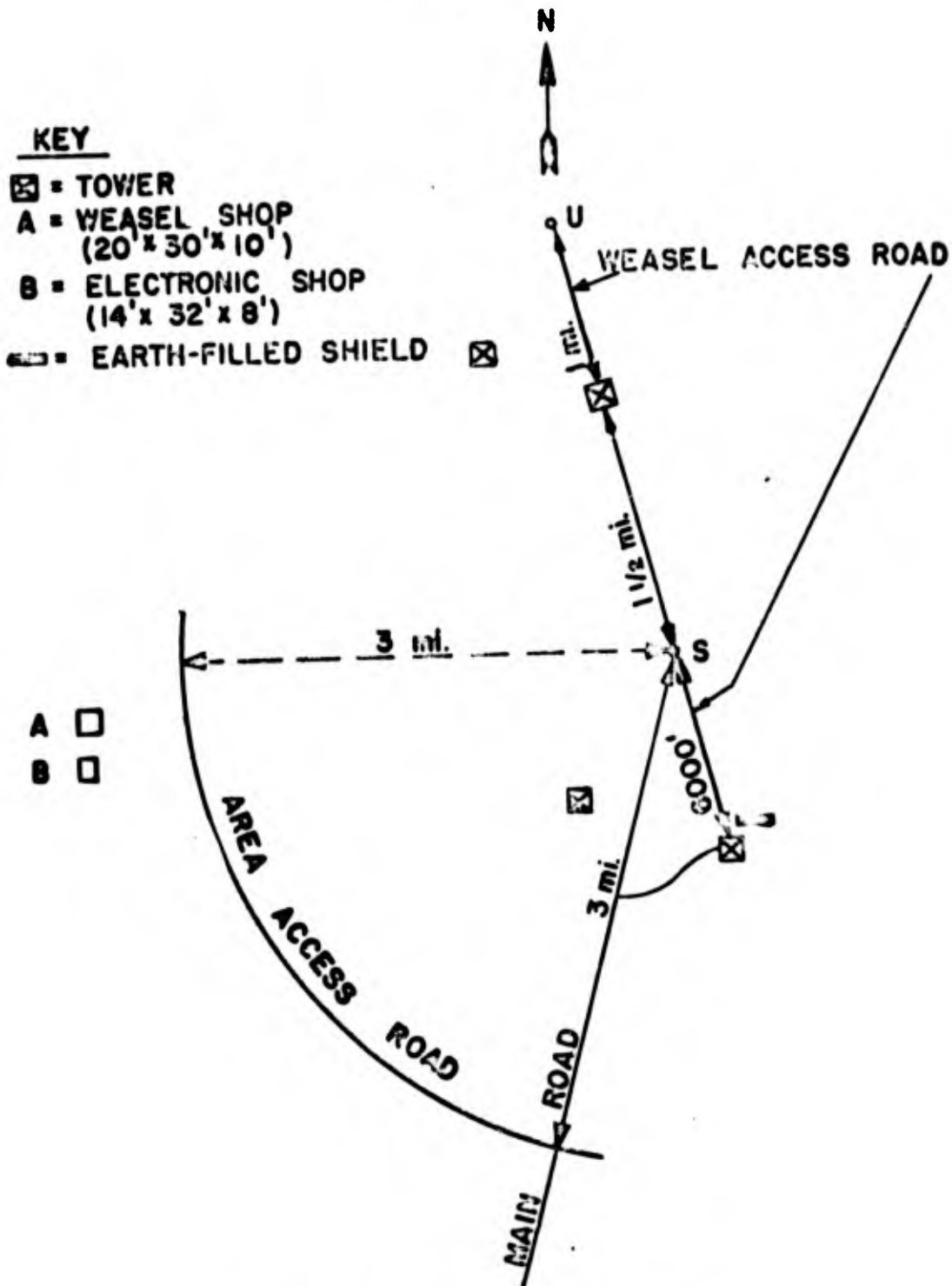
Fig. 1.1 Shop and Tower Layout
