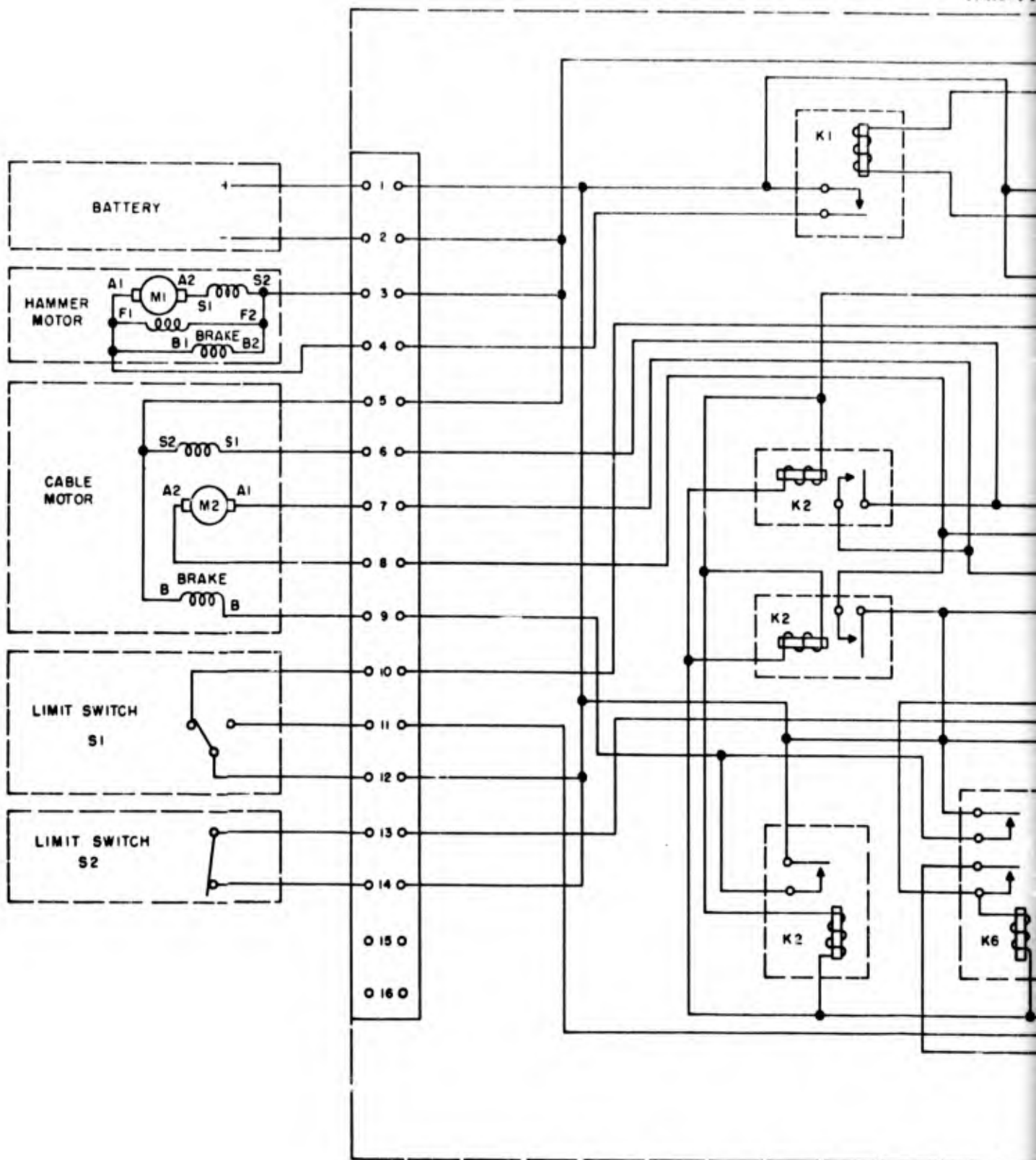
Figure 2.8 Schematic, Dec
