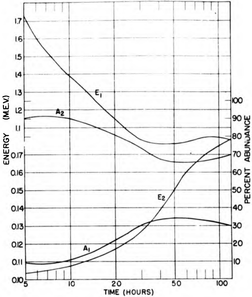
Figure 3.15. Effective Gamma Energies of Surface Soil Samples from Underground Burst
