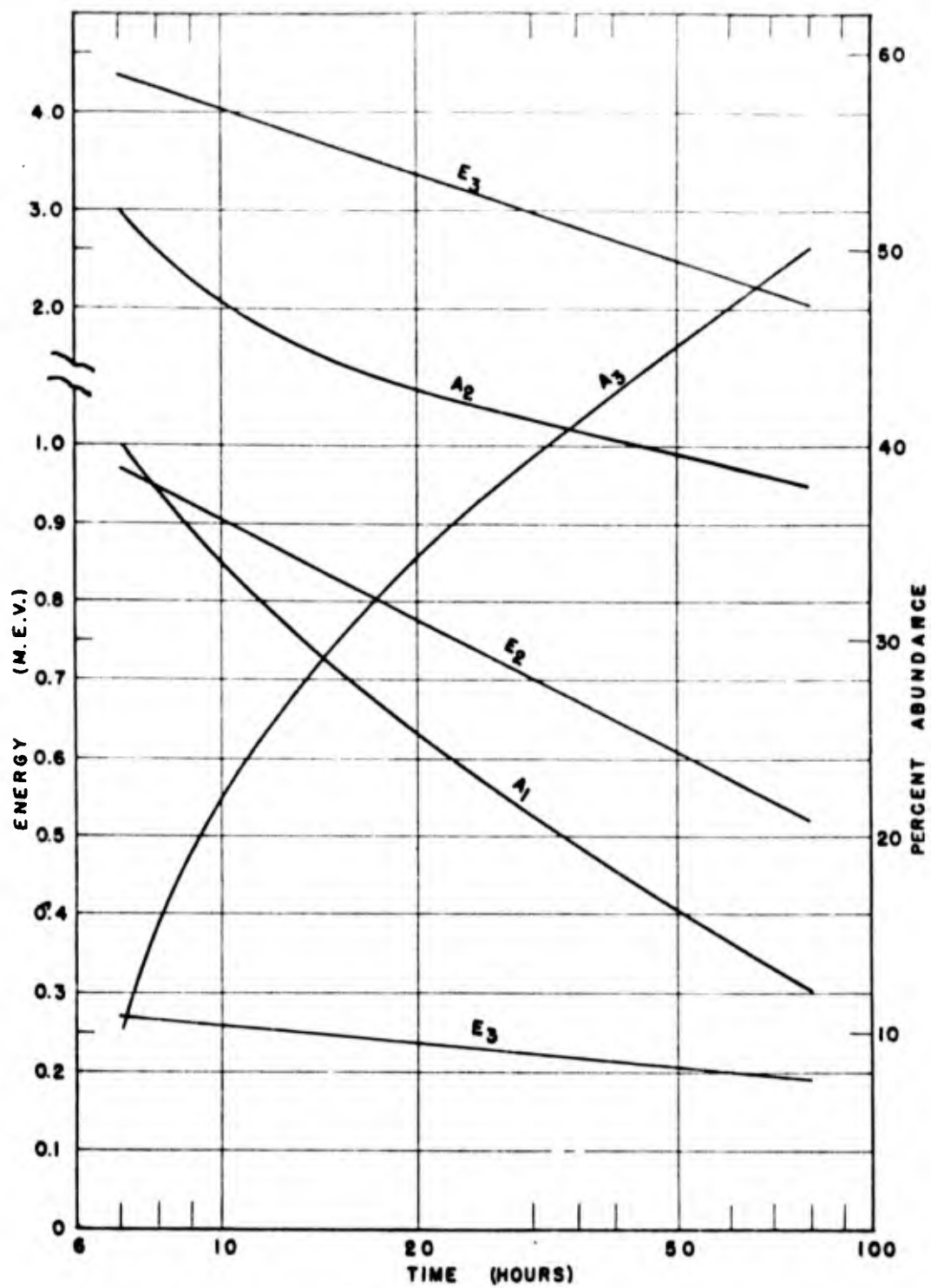
Figure 3.11. Effective Beta Energies of Surface Soil Samples from Surface Burst
