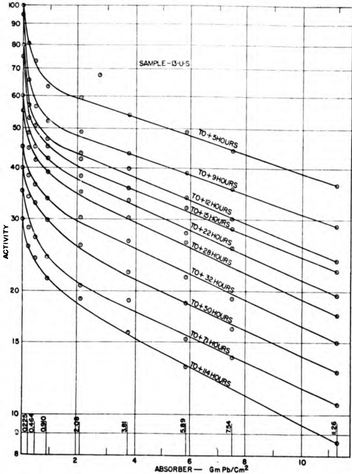
Figure 3.13. Typical Family of Lead Absorption Curves for Surface Soil Sample
