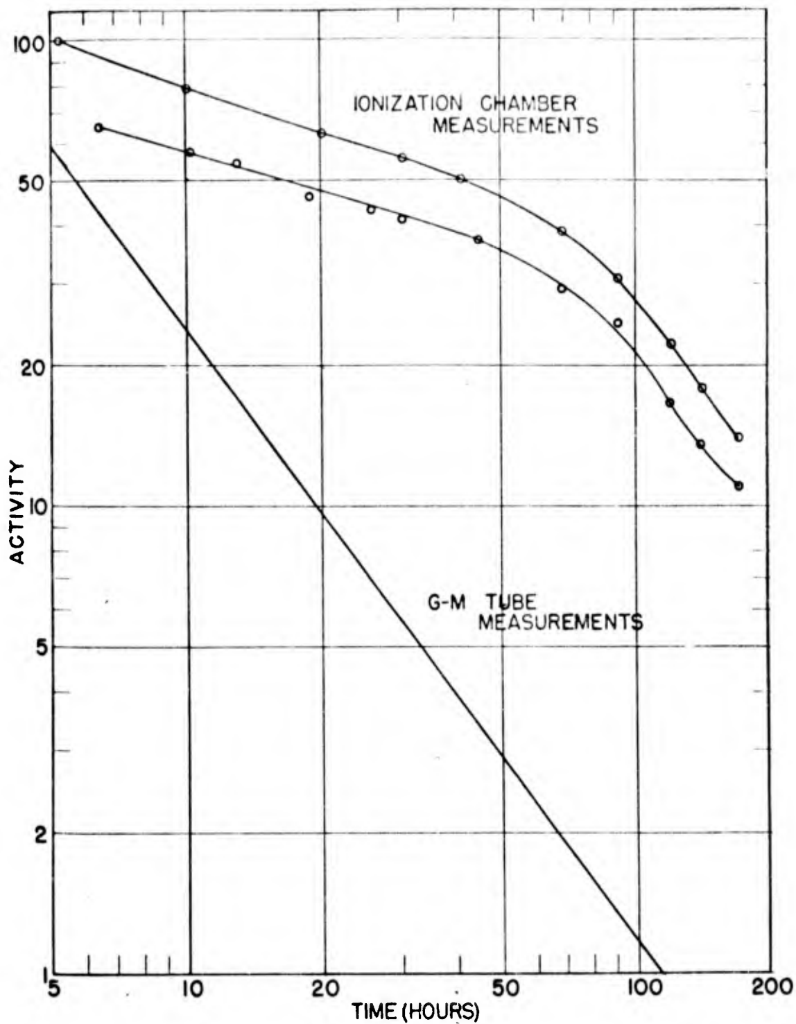
Figure 3.9. Ionization Chamber Measurements of Gamma Decay of Surface Soil Samples from Underground Burst
