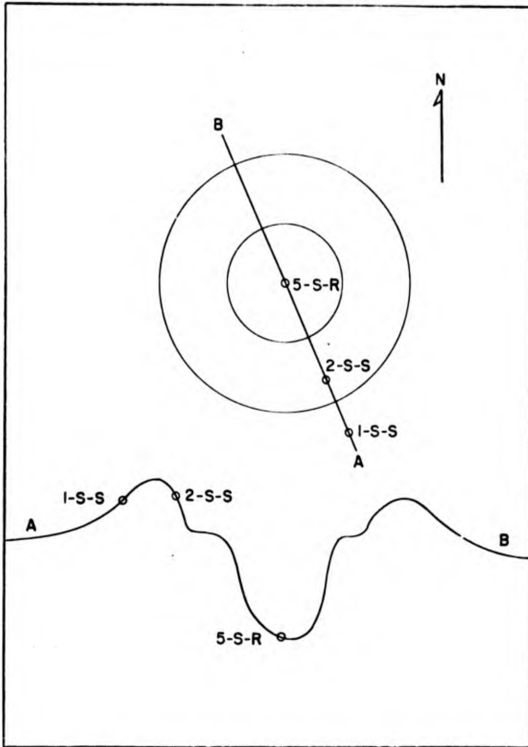
Figure 3.1. Location of Surface Samples on Crater of Surface Burst
