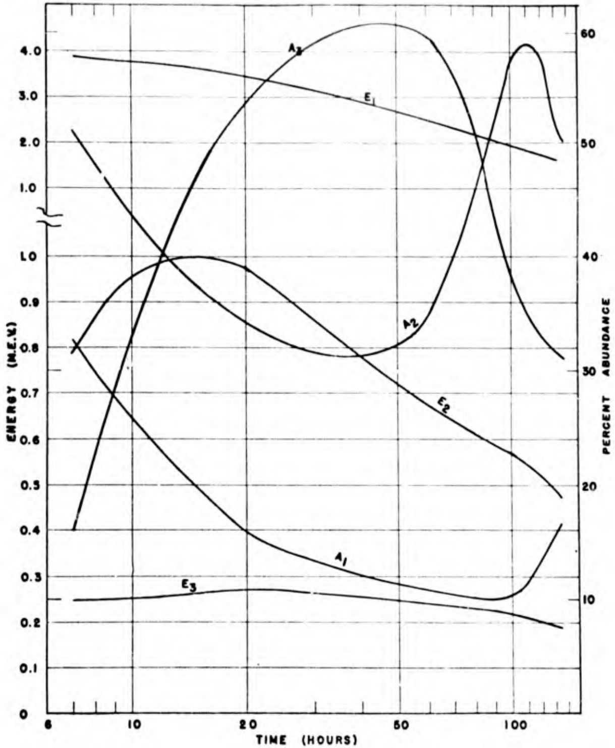
Figure 3.12. Effective Beta Energies of Surface Soil Samples from Underground Burst
