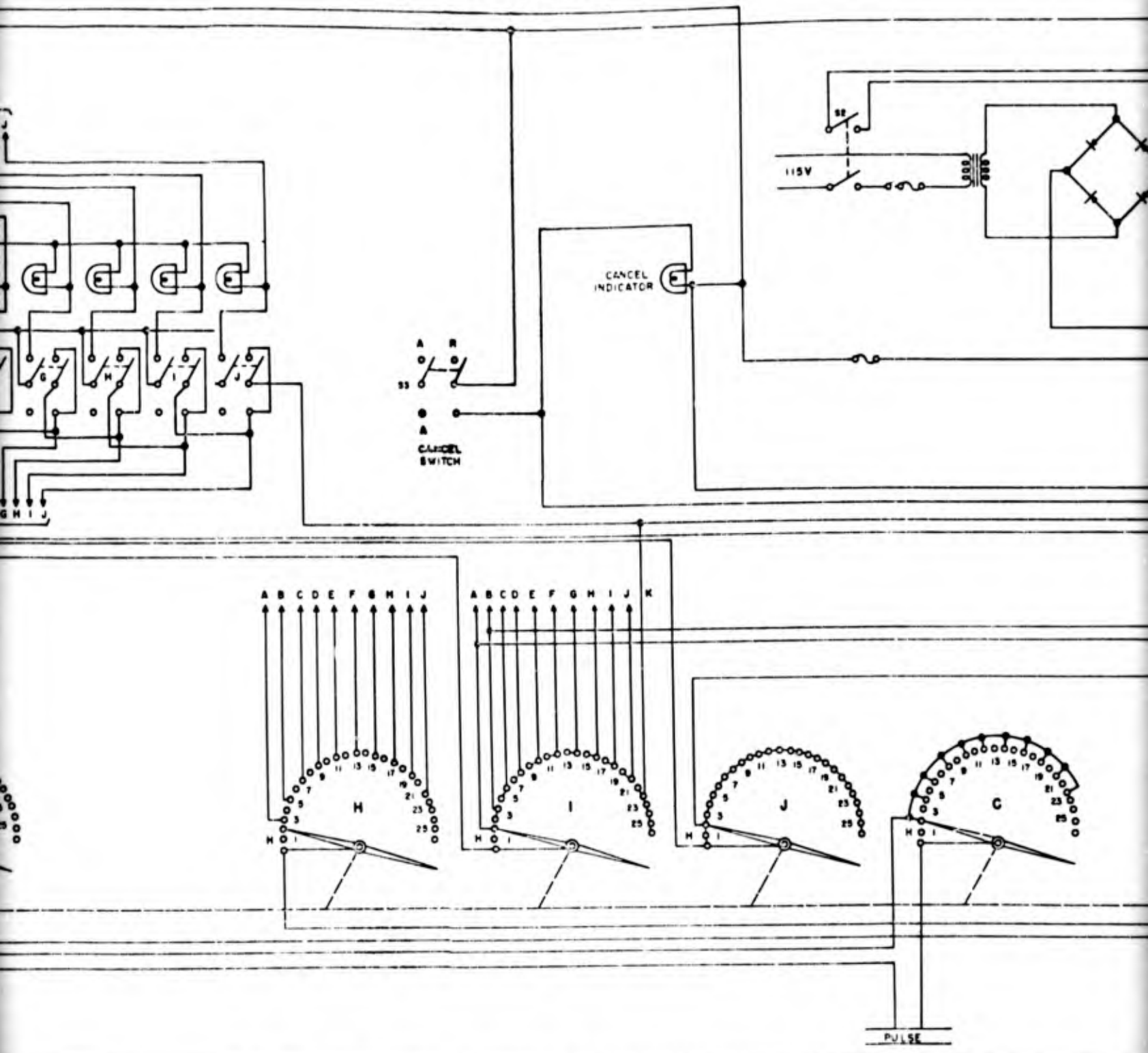
Figure 2.11 Schematic, Pulsed Scope Selector
