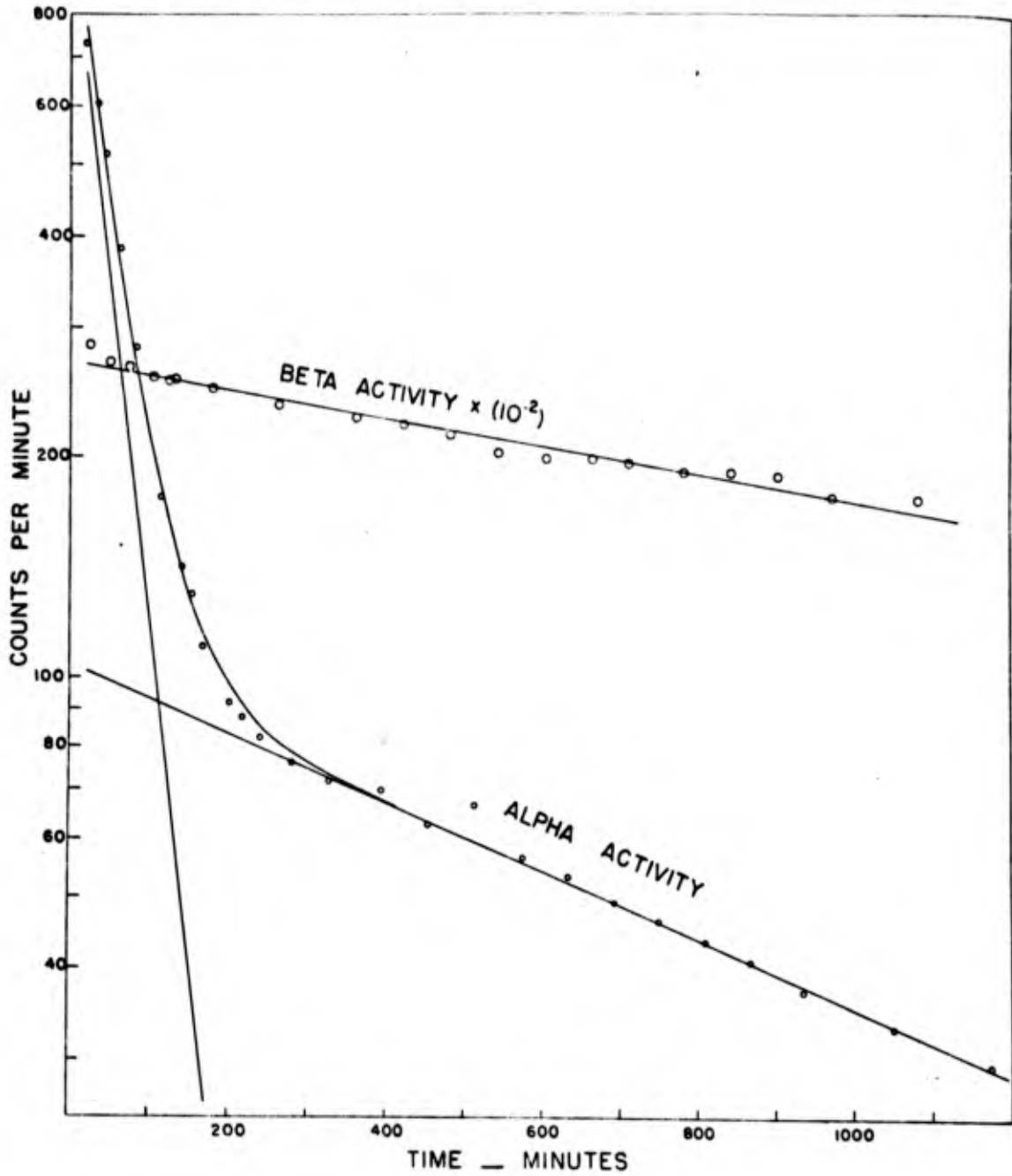
Figure B.1 Decay Curves of Airborne Radioactivity at Test Site
