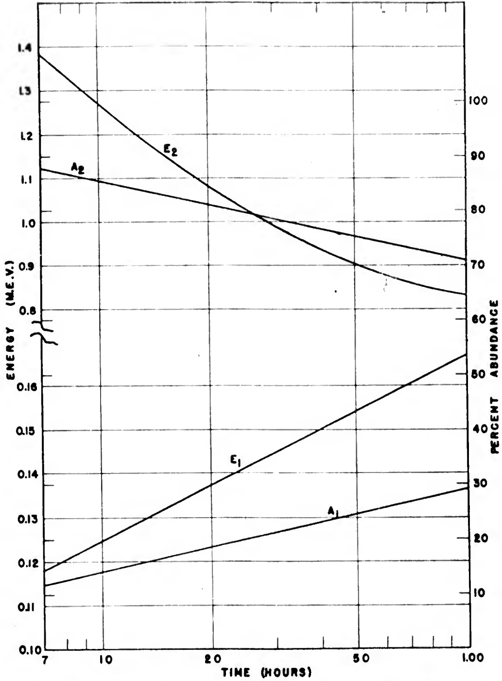
Figure 3.14. Effective Gamma Energies of Surface Soil Samples from Surface Burst
