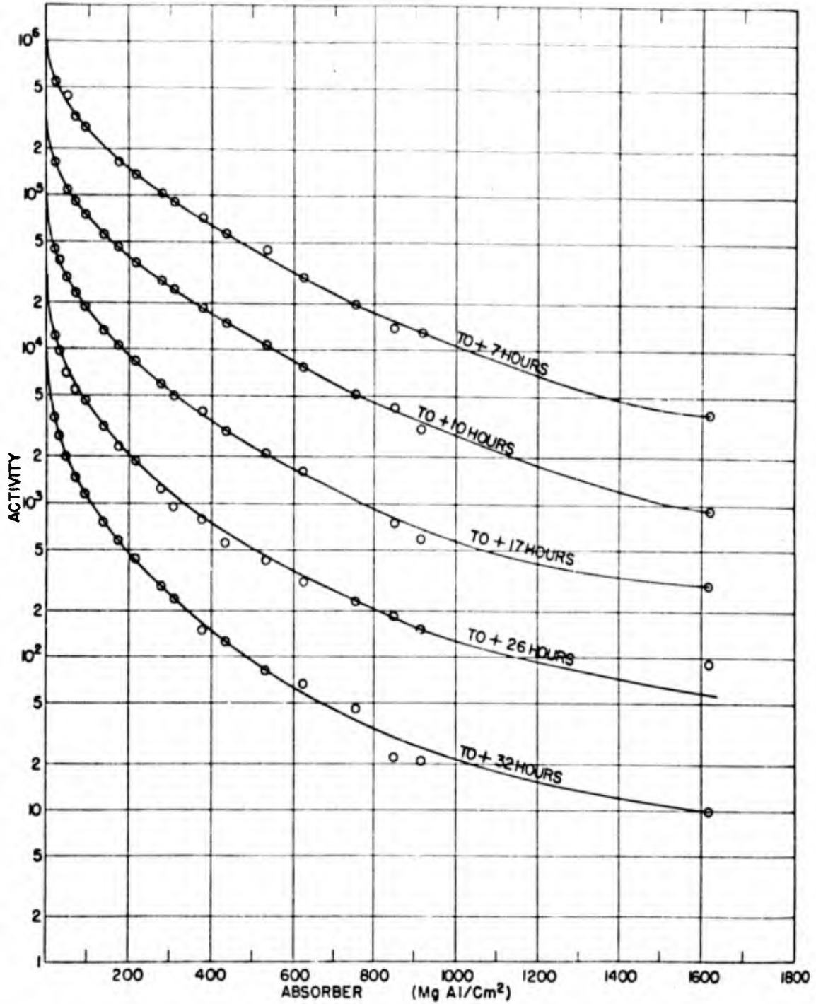
Figure 3.10. Typical Family of Aluminum Absorption Curves for Surface Soil Sample
