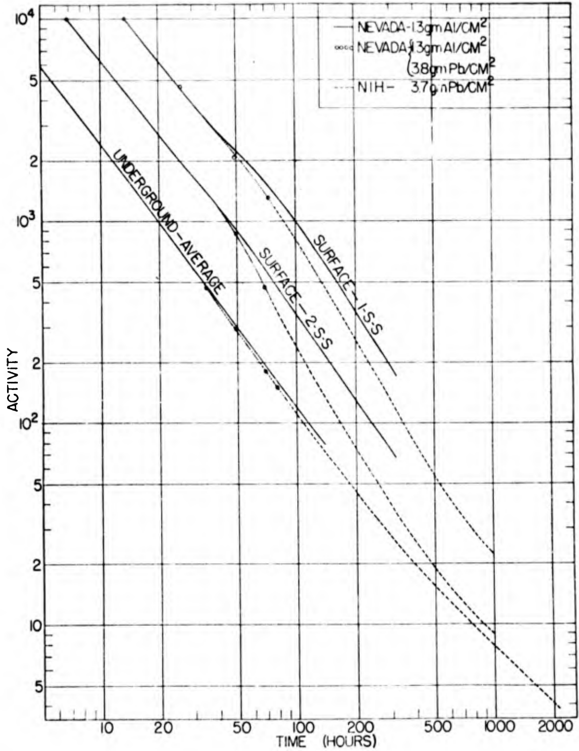
Figure 3.8. Geiger-Muller Tube Measurements of Gamma Decay of Surface Soil Samples.
