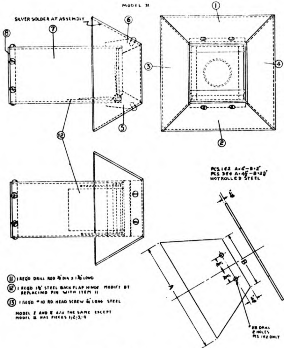
Figure 2.2 Details of sampling head
