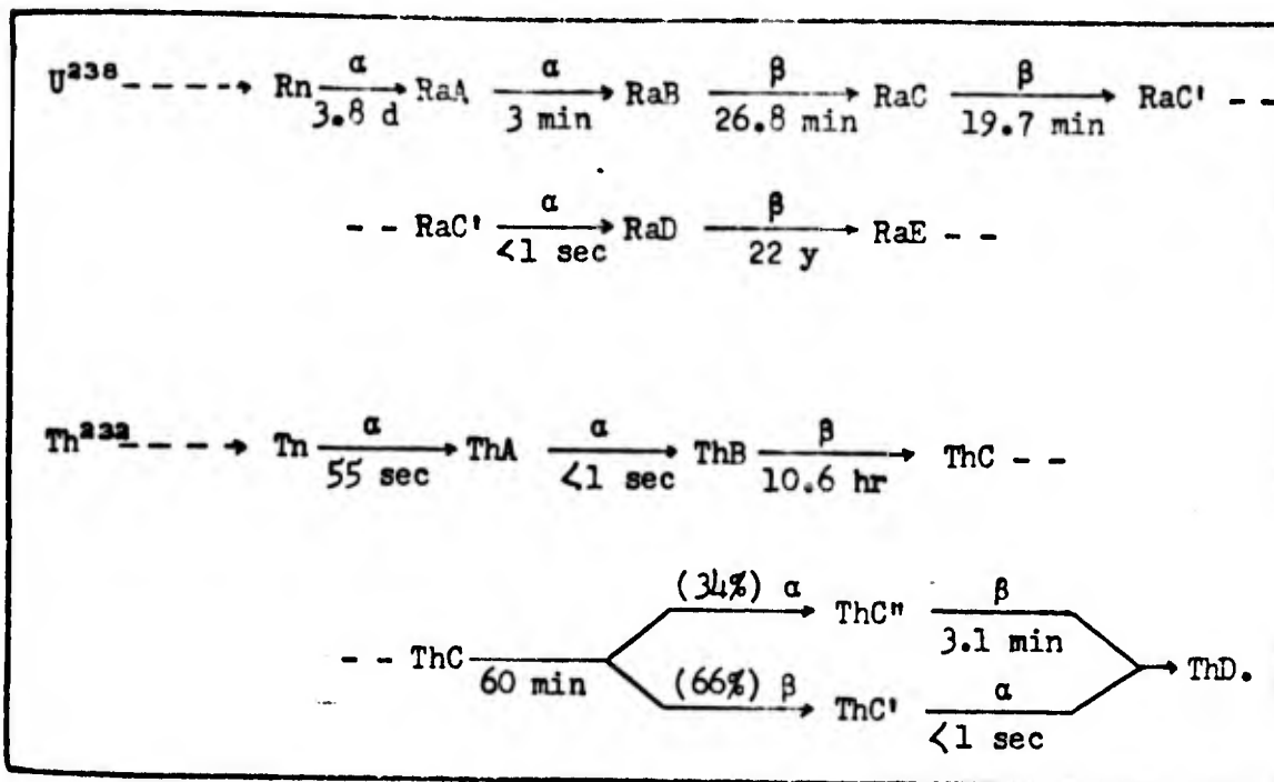
Figure B.2. Decay Schemes of Uranium 238 and Thorium 232
