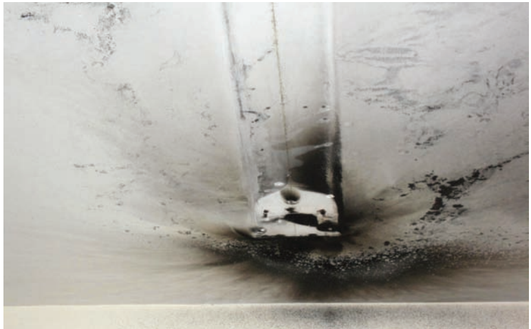
Unprotected high-voltage power cable wires exposed to leaking water.
