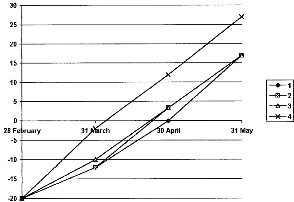
Figure 3. Soil temperature at depth 10 cm after different variants of snow cover destruction in spring in Yakutsk area: 1 - natural conditions, 2 - snow removal by use of black paint, 3 - mechanical snow removal, 4 - plastic mulch after mechanical snow removal.
