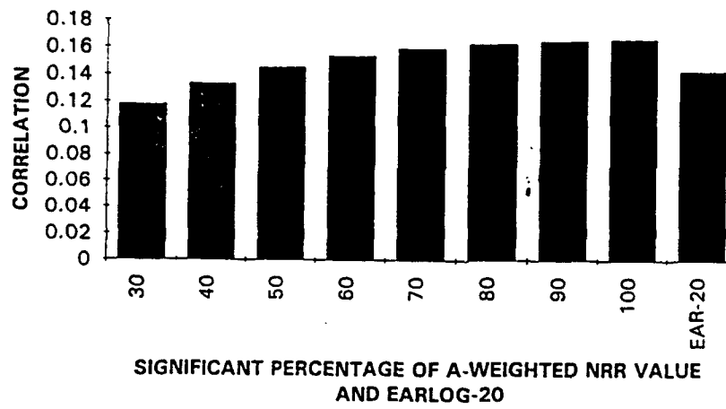
Figure 2 - Correlation between significant ( P < 0.05 ) Sound Exposure Level With Percent of A-Weighted NRR Value Correction, EARLOG-20 and Average Better Ear (1, 2, 3 and 4 kHz) In the Metal Fabricating Plant.
