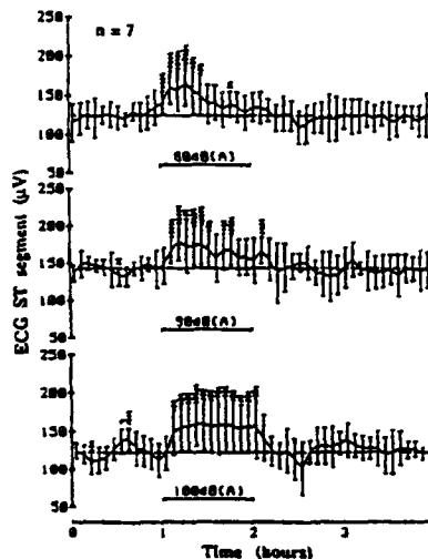
Fig 8. Effects of different sound pressure level noise exposure on the changes of ECG ST segment in type A male rats * p < 0.05 ** p < 0.01
