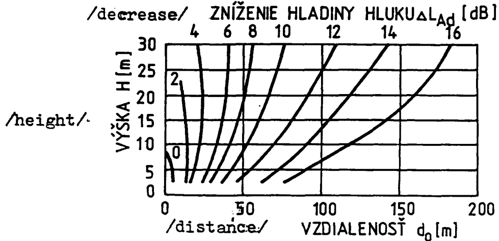
Fig.1 Noise level decrease in dependence on height and distance
