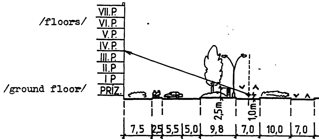
Fig.2 Cross section scheme of a road for measurement of traffic noise
