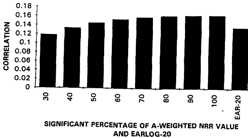
Figure 3 - Correlation between significant ( P < 0.05 ) Noise Immission With Percent of A-Weighted NRR Value Correction, EARLOG-20 and Average Better Ear (1, 2, 3 and 4 kHz) In the Metal Fabricating Plant.
