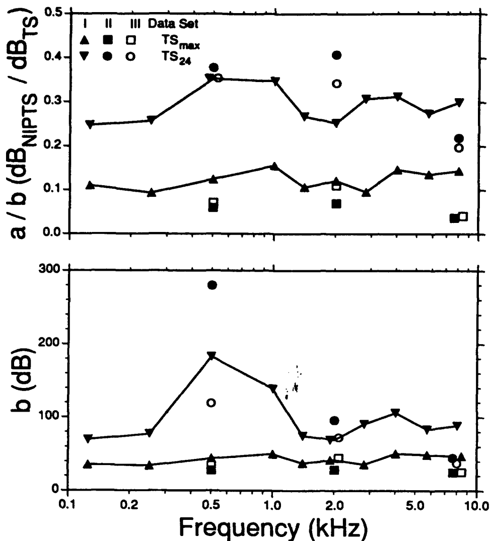
Figure 3. The values of the constants a and b derived from the exponential least-squares regression equations between TS_{max} or TS_{24} and NIPTS for all three data sets.
