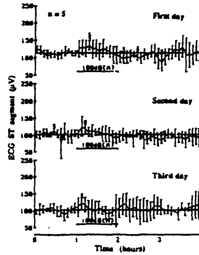
Fig 6. Effects of repeated noise exposure in three days on the noise stimulated changes of ECG ST segment in type B male rats * p < 0.05 ** p < 0.01
