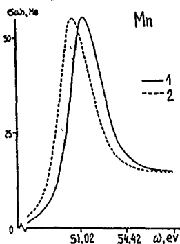
Fig.1. Mn M_{23} -photoabsorption cross section 1 -including and 2 - not including the potential D(\omega; r) . 3p level's spin-orbital split is neglected. \Gamma_{3p} = 3,0 \text{ eV} / 2 .
