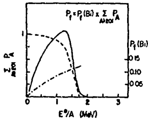
Fig. 2 Probabilities to form nuclei with mass number above 200 calculated with the multifragmentation model of ref. 1 (dashed curve). The solid curve shows the fission probabilities after multifragmentation, assuming the residual nuclei fission with the same energy dependence as Bi. The dot-dashed curve shows the fission probabilities calculated for Bi using a standard code 3) .
