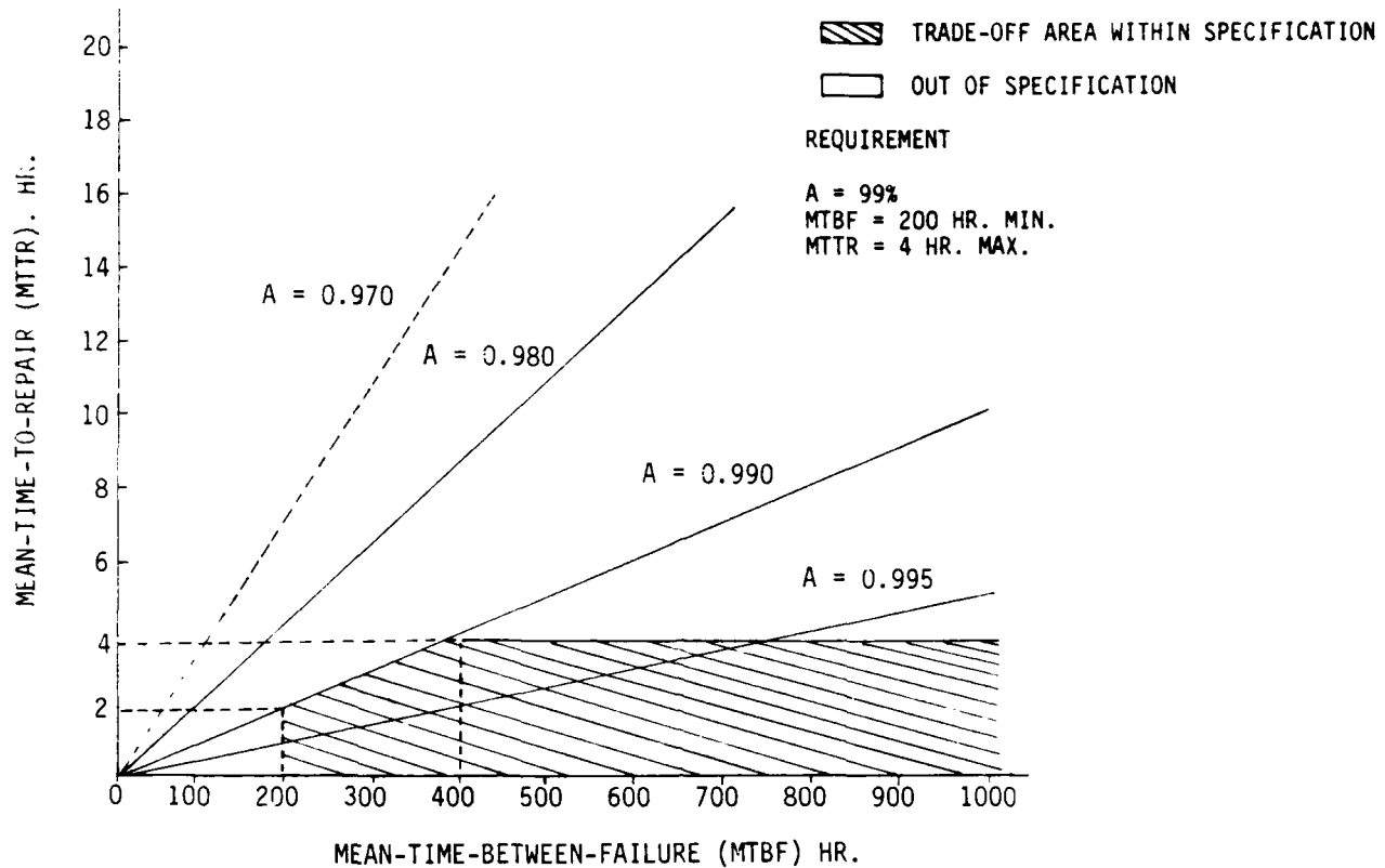
FIGURE 14.4: RELIABILITY-MAINTAINABILITY TRADE-OFFS
