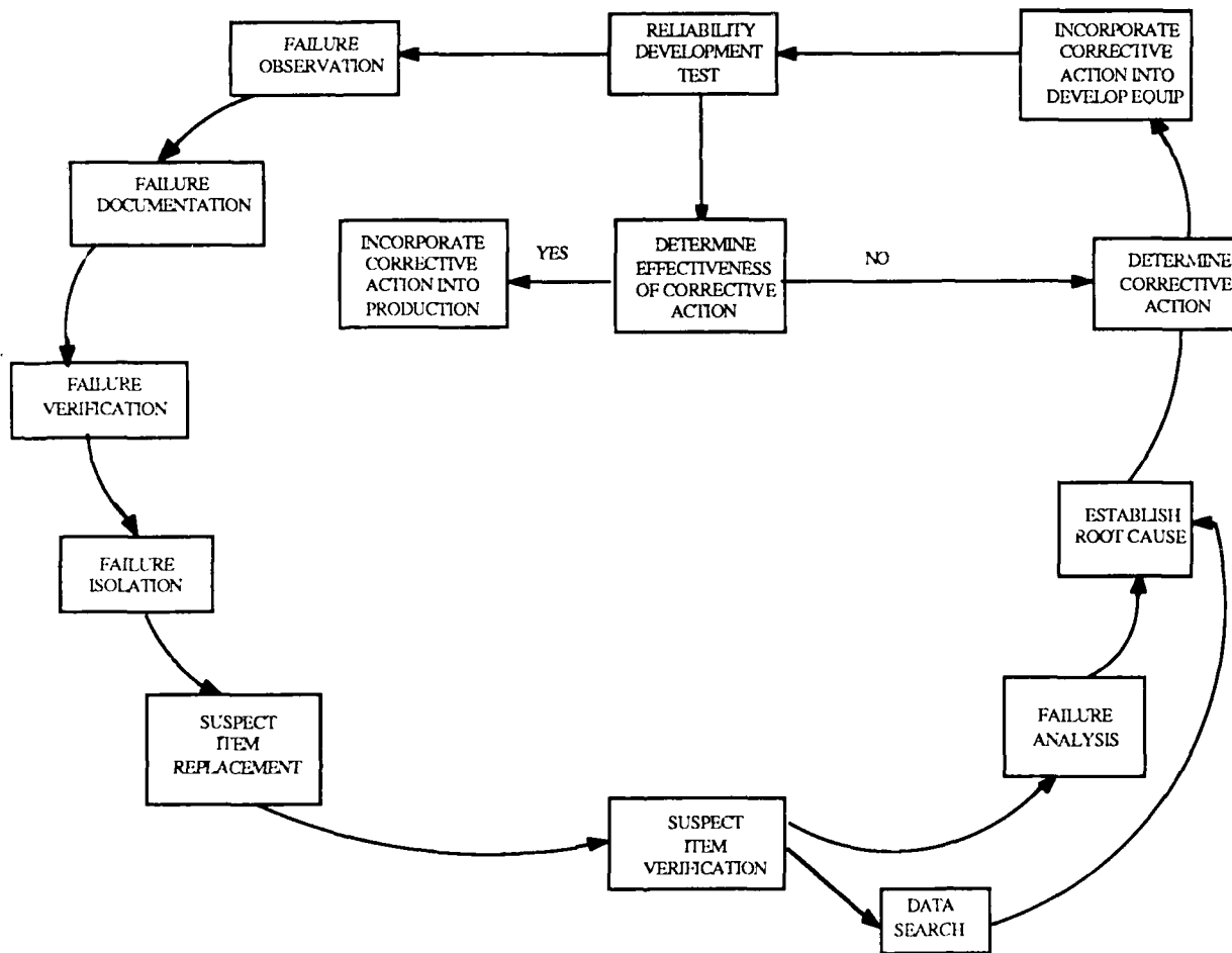
FIGURE 6.1: CLOSED LOOP FAILURE REPORTING AND CORRECTIVE ACTION SYSTEM
