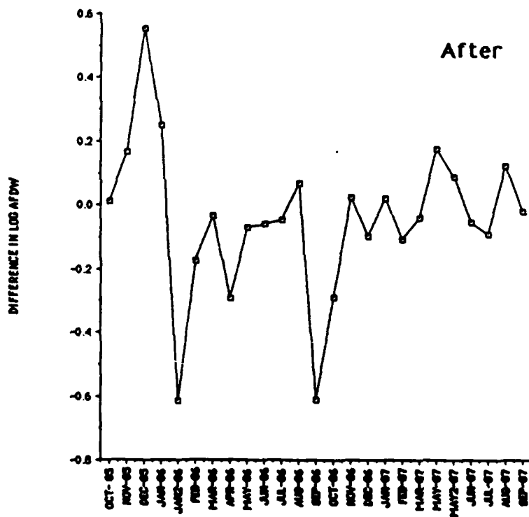
Figure 2.12 Organic Matter Biomass (AFDW) Differences Between Sites for the Before and After Period.
