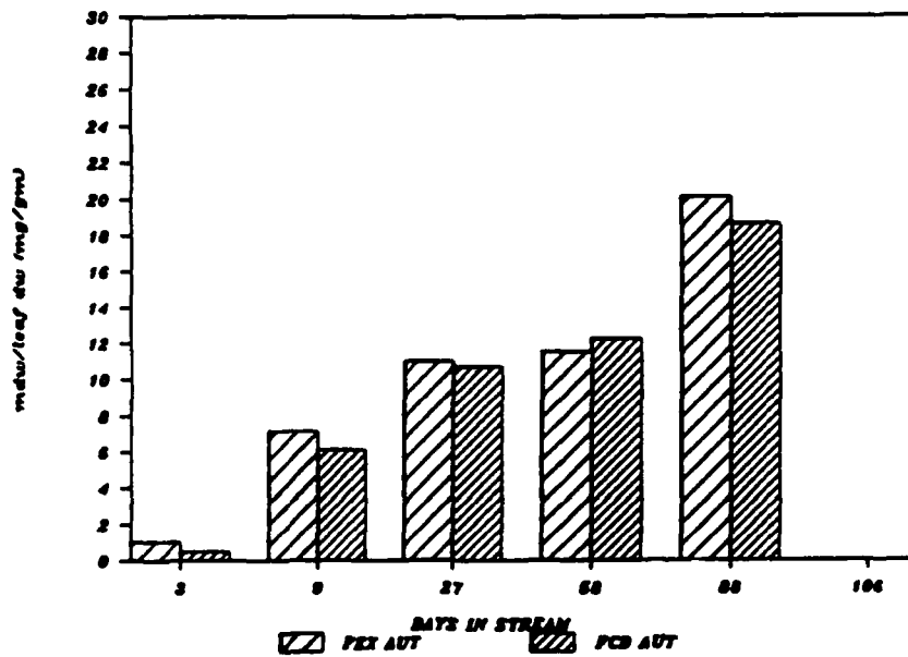
Figure 6.8A Total biomass of insects (adjusted to leaf mass) on fresh leaves for FEX and FCD sites.
