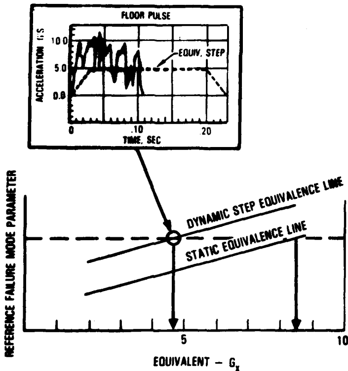
B. L1649 CRASH TEST FLOOR PULSES IN THE LONGITUDINAL AFT DIRECTION (FORWARD INERTIA) ARE LESS THAN 98 STATIC AND EQUIVALENT TO < 68 DYNAMIC STEP PULSE
