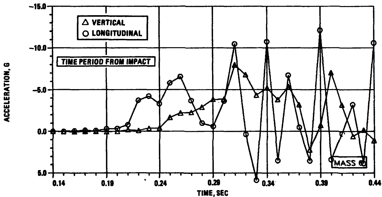
Figure 5-11. - Airframe responses, ground-to-ground overrun GGO-328-3.
