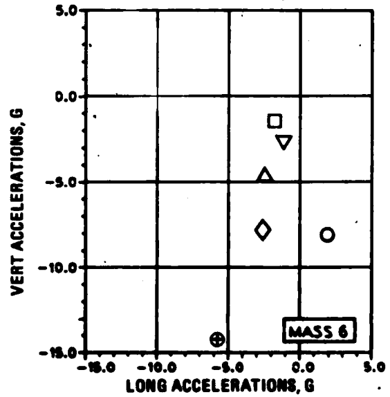
Figure 9-5. Simultaneous Accelerations, Ground-To-Ground Symmetrical Overruns
