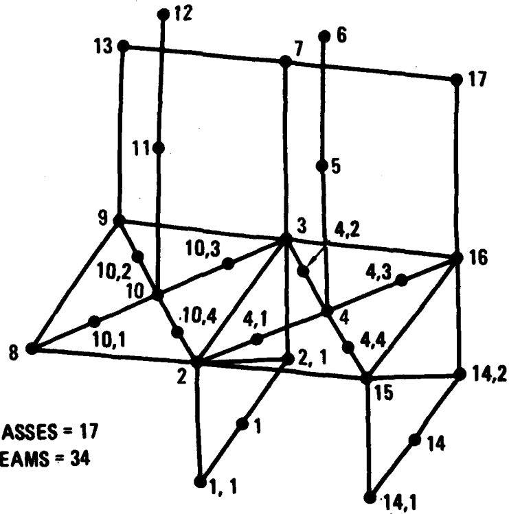
Figure 4-7. Two passenger seat/occupant model.
