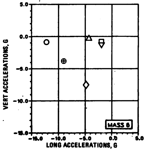
Figure 9-5. Simultaneous Accelerations, Ground-To-Ground Symmetrical Overruns
