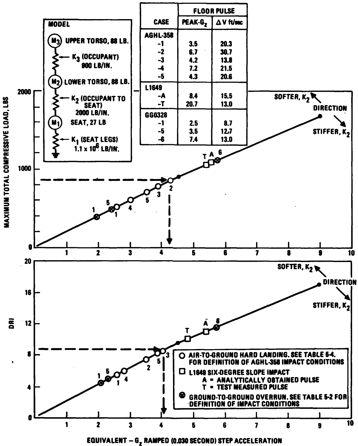
Figure 8-12. Equivalent -G 2 Ramped Step Input for Analytically Obtained Hard Landing Pulses
