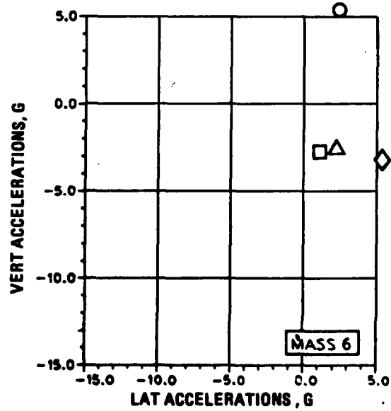
Figure 9-7. Simultaneous Accelerations, Unsymmetrical Impact Conditions
